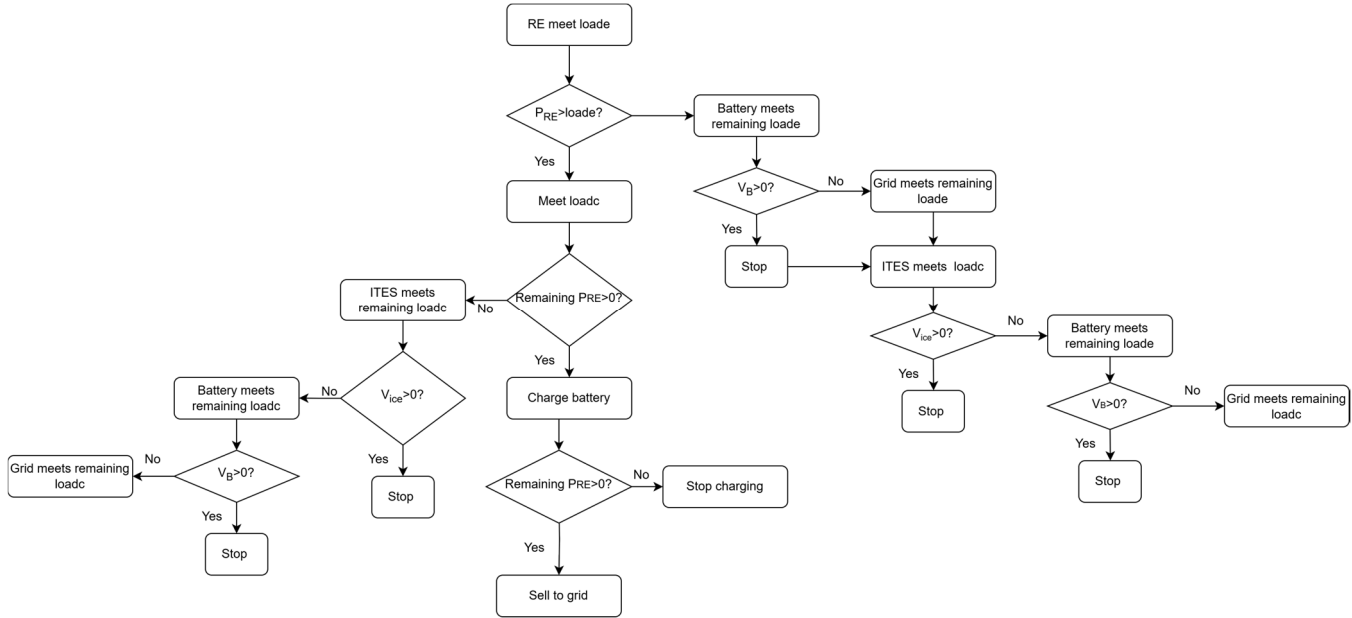
Figure 2. Operational logic diagram.
