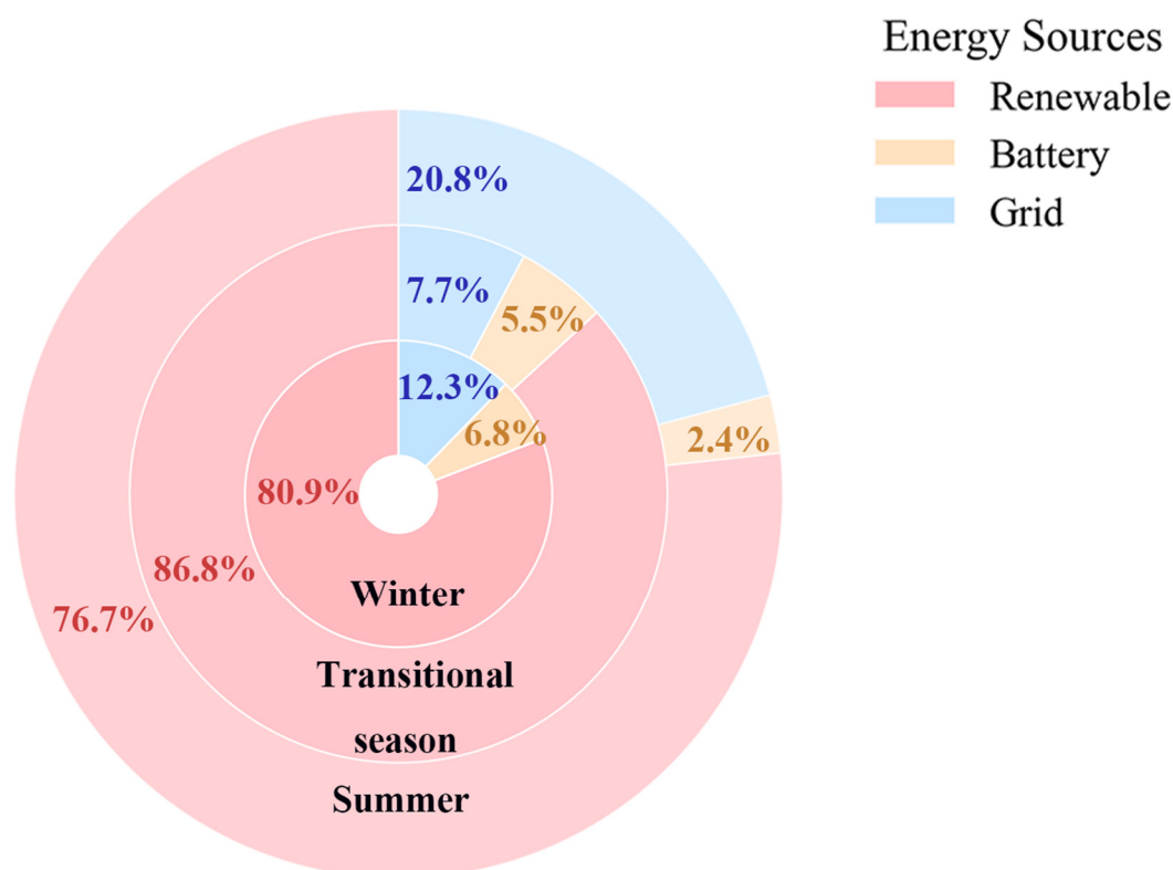
Figure 16. Seasonal energy mix composition.
