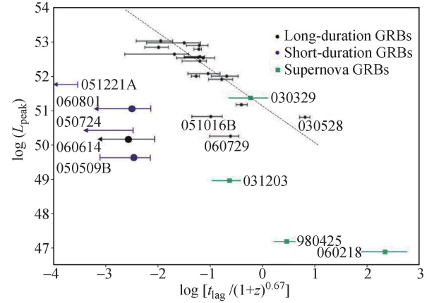
Fig. 6 Spectral lag as a function of peak luminosity showing GRB 060614 in the region of short-duration GRBs [68].
