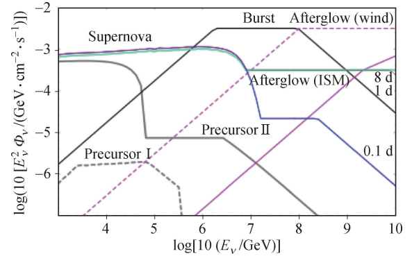
Fig. 15 Predicted neutrino fluxes from a relatively nearby GRB 030329 at a redshift z = 0.17 . An accompanying supernova was detected from this long GRB as well. Reproduced from Ref. [179].
