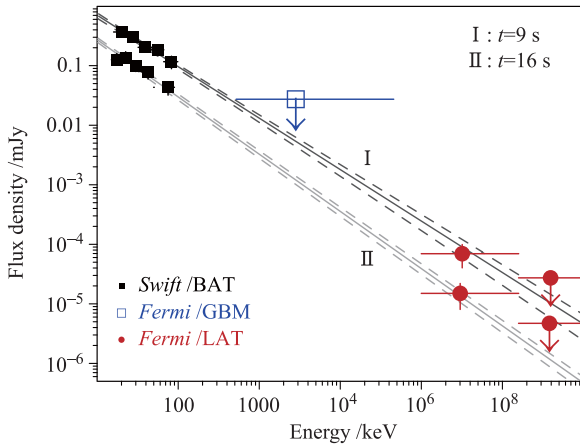
Fig. 14 Broadband spectra of GRB 110731A at two time intervals after the trigger. Single power laws fitting the spectra, together with flux decay behavior in Fig. 13 imply that LAT emission is afterglow. Reproduced from Ref. [138].
