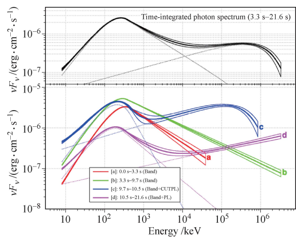
Fig. 8 Prompt emission spectra of GRB 090926A at different time intervals (bottom panel) as well as during the entire prompt phase (top panel). A power-law component in addition to the Band spectrum, as also found in other bright LAT-detected GRBs, is required to fit the spectra. A cutoff in the PL component at few GeV has been detected in this GRB and in GRB 110731A [138]. Reproduced from Ref. [26].
