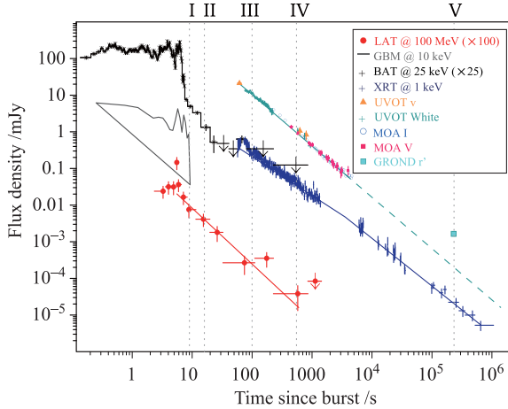
Fig. 13 Multiwavelength light curves of GRB 110731A from Fermi GBM and LAT; Swift BAT, XRT and UVOT; and ground-based optical telescopes. Smooth decay of the fluxes across the wavelengths after \sim 6 s suggests their origin, including LAT emission, as from a decelerating blast wave in stellar wind environment. Reproduced from Ref. [138].
