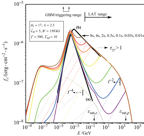
Fig. 9 Proton-synchrotron radiation model for delayed onset of LAT emission in GRB 080916C. The delay is caused by a build-up of proton-synchrotron flux and a shift of cooling frequency from very high energies to the LAT range, with time. GBM radiation is assumed to be dominated by electron-synchrotron radiation. Reproduced from Ref. [143].
