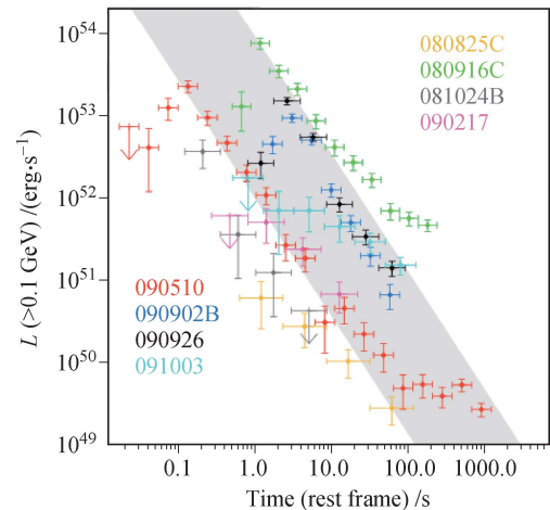
Fig. 11 Light curves of \gtrsim 100 MeV radiation from a few LAT-detected GRBs, which show decaying LAT flux as a common feature. The grey band with slope t^{-10/7} is the expected decay behavior for afterglow emission from a radiative blast wave. Reproduced from Ref. [151].
