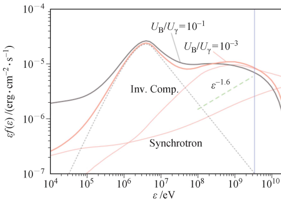
Fig. 10 Photohadronic cascade radiation model for the additional power-law component detected in GRB 090510. Synchrotron radiation from charged pions, muons and e^+e^- contribute to the observed spectra. High-energy neutrinos are also expected in this model. Reproduced from Ref. [144].
