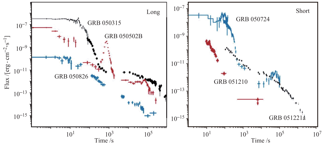
Fig. 1 Representative examples of X-ray afterglows of (a) long and (b) short Swift events with steep-to-shallow transitions (GRB 050315, GRB 050724), large X-ray flares (GRB 050502B, GRB 050724), and rapidly declining (GRB 051210) and gradually declining (GRB 051221a, GRB 050826; flux scale divided by 100 for clarity) afterglows. Reproduced from Ref. [12].
