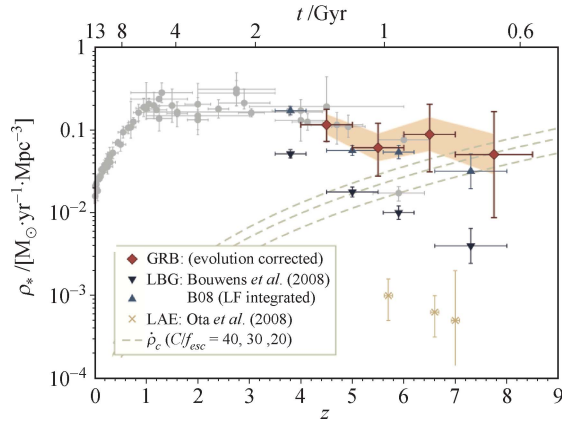
Fig. 5 Cosmic star formation history. Shown are the data compiled in Hopkins & Beacom [40] (light circles) and contributions from Ly emitters (LAE) [41]. Recent LBG data are shown for two UV LF integrations: down to 0.2L_* (down triangles; as given in Bouwens et al. [42]) and complete z = 3 (up triangles). Swift GRB-inferred rates are diamonds, with the shaded band showing the range of values resulting from varying the evolutionary parameters. Also shown is the critical density derivative from Madau et al. [43] for C/f_{esc} = 40, 30, 20 (dashed lines, top to bottom). Reproduced from Ref. [38]. See also study by Robertson & Ellis [39].
