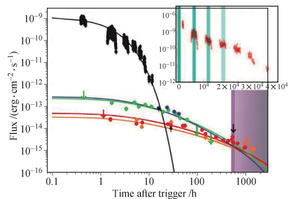
Fig. 7 Light curves of GRB 101225 in five energy bands: X-rays at 1 keV (black), UV at 2030 angstroms (green) and 2634 angstroms (blue), and optical at 6400 angstroms ( R band, red) and 7700 angstroms ( I band, orange) [93]. The inset (with t in seconds) shows the Swift/XRT light curve. Shaded regions highlight the periastron passages calculated using a tidal disruption model [93].
