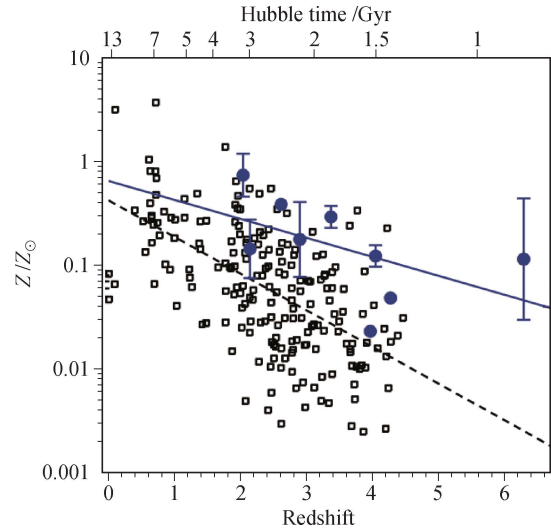
Fig. 4 Redshift evolution of the metallicity (represented here by the ratio of oxygen to hydrogen abundance) relative to solar values, for GRBs shown with blue dots and active galaxy quasars shown with open circles. The abundances are determined from spectral absorption lines in the continuum radiation. GRB lines are predominantly from the gas in the host galaxy in the star-forming region near the explosion, whereas quasars are of random lines-of-sight through the galaxy. The GRB metallicity is on average \sim 5 times larger than in QSO. These are based on damped Lyman alpha (DLA) spectral features. The upper horizontal x -axis indicates the age of the Universe (Hubble time). Reproduced from Ref. [36].
