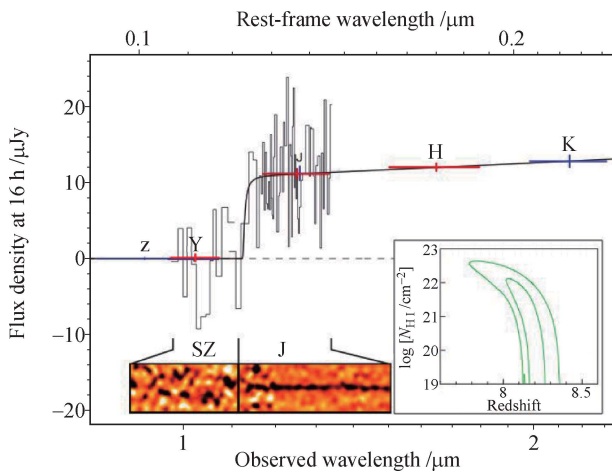
Fig. 3 The composite spectrum of the GRB 090423 afterglow obtained with the VLT. Also plotted are the sky-subtracted photometric data points obtained using Gemini North & South and VLT. A model spectrum showing the H I damping wing for a host galaxy with a hydrogen column density of N_{\text{HI}} 5 \times 10^{21} \text{ cm}^{-2} at a redshift of z = 8.23 is also plotted (solid black line). Inset, allowing for a wider range in possible host N_{\text{HI}} values gives the 1\sigma (68%) and 2\sigma confidence contours shown. Reproduced from Ref. [33].
