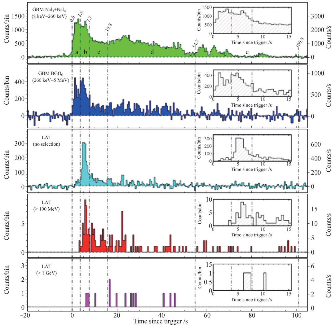
Fig. 2 Light curves of GRB 080916C with GBM (top three panels) and LAT (bottom two panels). The high energy LAT emission is delayed relative to the lower energy GBM emission. Reproduced from Ref. [22].
