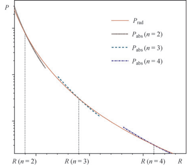
Fig. 3 Radiated power P_{\text{rad}} [ 10^{-7} \text{ J} \cdot \text{s}^{-1} ] and absorbed power P_{\text{abs}} [ 10^{-7} \text{ J} \cdot \text{s}^{-1} ] vs radius R [cm] of the electron circular orbit. For any number n of plane orbits (in QM terms, n is the principal quantum number) there is a stable point of intersection P_{\text{abs}}(n, R) = P_{\text{rad}}(n) if the average effect of the zero-point field (ZPF) is considered. The ZPF fluctuations concordant with the radiation damping cause the transition from n to n - 1 .
