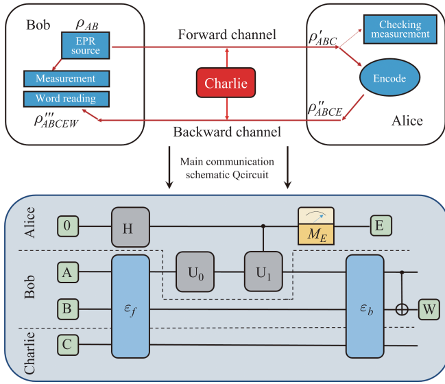
Fig. 1 Schematic of quantum secure direct communication and the main communication quantum circuit. The lower part is used as an illustration of the main communication process. H is a Hadamard gate; U_0 and U_1 are the encoding unitary gates; M_E is the post-selection measurement selected by Alice to encode classical information; 0 denotes state |0\rangle while A , B , C , E , W denote the corresponding registers: A , the qubit that Bob transmits to Alice; B , the qubit Bob possesses at his laboratory; C , the adversary's system (needless to be a qubit system); E , the register storing encoding information of Alice; W , the register storing Bob's decoding information. Here the entanglement state \rho_{AB} = (|00\rangle + |11\rangle)/\sqrt{2} .
