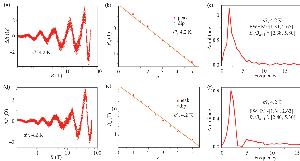
Fig. 2 Reproducible log-periodic oscillations in different ZrTe 5 samples. (a–c) log-periodic oscillations, index plot, FFT results for sample #7 at 4.2 K. (d–f) log-periodic oscillations, index plot, FFT results for sample #9 at 4.2 K. Reproduced from Ref. [13].
