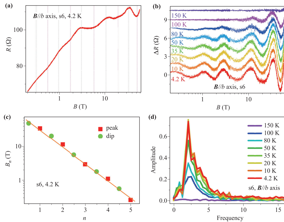
Fig. 1 Log-periodic MR oscillations in ZrTe 5 . (a) MR behavior of sample #6 in an ultrahigh magnetic field up to 58 T at 4.2 K. Dotted lines serve as guides to the eye. (b) MR oscillations in s6 after subtracting a smooth background from the raw data. (c) Index plot for the log-periodic oscillations. (d) FFT results for the MR oscillations at different temperatures in the form of \Delta R versus \log(B/B') with B' = 1 T. Reproduced from Ref. [13].
