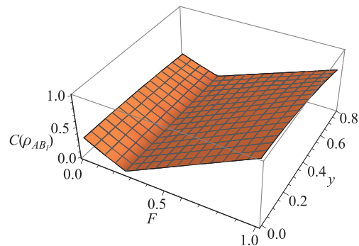
Fig. 3 A plot of C(\rho_{AB_I}) as function of acceleration parameters y and F .
