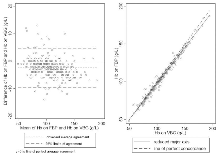
Figure 1. Agreement for full range of Hb values
