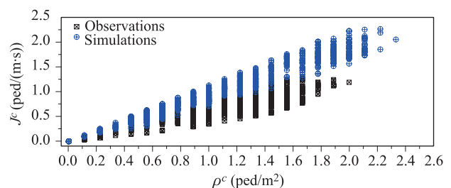
Fig. 3 Comparisons of fundamental diagrams of observations and simulation data obtained using Helbing's model.
