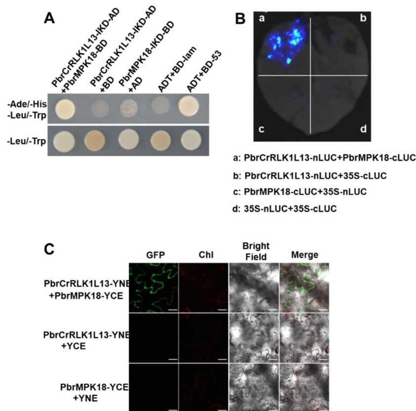
Fig. 5 PbrMPK18 interacts with PbrCrRLK1L13. A PbrMPK18 interacts with the intracellular domain of PbrCrRLK1L13 in yeast two-hybrid assays. The intracellular domain of PbrCrRLK1L13 fused to the pGADT7 vector and that of PbrMPK18 fused to the pGBKT7 vector. Growth in the medium that lacked Trp, Leu, His, and Ade indicated protein–protein interactions. B PbrMPK18 and PbrCrRLK1L13 interact in the plasma membrane of N. benthamiana leaf epidermal cells in the LCI assay. Fluorescence on the leaf surface indicated protein–protein interactions. C PbrMPK18 and PbrCrRLK1L13 interact in the plasma membrane of N. benthamiana leaf epidermal cells in the BiFC assay. The GFP signal indicates the interaction between PbrMPK18 and PbrCrRLK1L13. Chl represents chloroplast autofluorescence. Merge represents the merged image of GFP, Chl, and bright field. Scale bars = 5 \mu m
