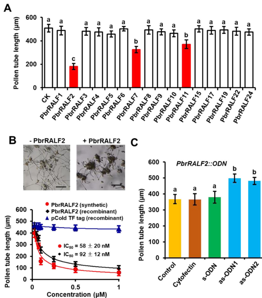
Fig. 1 PbrRALFs inhibit pollen tube growth. A Pollen tubes from pear were treated with 1 μM recombinant PbrRALFs, and pollen tube growth was measured. Selected PbrRALFs were expressed in pollen by RT-PCR (Supplementary Fig. S1A). Different letters indicate significant differences, as determined by one-way ANOVA ( P < 0.05 , n = 3 ). Three independent experiments were conducted. Data points are presented as the means \pm s.e.m., with those significantly different from the control (CK) shown in red. B Recombinant or synthetic PbrRALF2 at different concentrations (0.025 μM, 0.05 μM, 0.075 μM, 0.1 μM, 0.25 μM, 0.5 μM, and 1 μM) was added to precultured pollen tubes. Images shown were acquired 10 h after treatment without or with purified recombinant PbrRALF2. Scale bars = 0.1 mm. Data points are presented as the means \pm s.e.m. ( IC_{50} = 58 \pm 20 nM for synthetic PbrRALF2 and 92 \pm 12 nM for recombinant PbrRALF2). C Knockdown (antisense oligodeoxynucleotide; as-ODN) of the expression of PbrRALF2 promoted pollen tube growth ( P < 0.05 , n = 3 ), whereas s-ODN (sense ODN) and cytofection control had no function. UT indicates no treatment controls. Different letters indicate significant differences, as determined by one-way ANOVA ( P < 0.05 , n = 3 ). Three independent experiments were conducted
