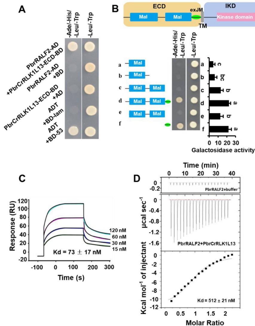
Fig. 2 Binding of PbrRALF2 to PbrCrRLK1L13. A PbrRALF2 interacts with the extracellular domain of PbrCrRLK1L13 in yeast. PbrRALF2 was fused to the pGADT7 vector, and the extracellular domain of PbrCrRLK1L13 was fused to the pGBKT7 vector. Growth in the medium that lacked Trp, Leu, His, and Ade indicated protein–protein interactions. B Extracellular juxtamembrane (exJM) region of PbrCrRLK1L13 is required for the PbrRALF2 interaction. The predicted structure of PbrCrRLK1L13, including the extracellular domain (ECD), exJM, transmembrane domain (TM), and intracellular kinase domain (IKD). Dissection of the exJM region of PbrCrRLK1L13 is required for the interaction with PbrRALF2 in a yeast two-hybrid assay. The interaction strength was quantified through \beta -galactosidase activity. Different letters indicate significant differences, as determined by one-way ANOVA ( P < 0.05 , n = 3 ). C Binding of four concentrations of PbrRALF2 to PbrCrRLK1L13 in the surface plasmon resonance (SPR) assay. Different colored lines represent the titration of different concentrations of PbrRALF2 protein in the SPR assay. The light blue line indicates the 120 nM PbrRALF2 assay, the pink line indicates the 60 nM PbrRALF2 assay, the dark blue line indicates the 30 nM PbrRALF2 assay, and the green line indicates the 15 nM PbrRALF2 assay. The black lines represent the fitting line. The solid line is a fit with Michaelis–Menten kinetics, yielding an apparent dissociation constant of K_d = 73 \pm 17 nM. D Quantitative binding analysis using PbrRALF2 and the extracellular domain of PbrCrRLK1L13 using isothermal titration calorimetry (ITC). A representative thermogram was obtained from 200 \mu M PbrRALF2 titrations into 20 \mu M PbrCrRLK1L13. Nonlinear regression of the PbrRALF2 vs. PbrCrRLK1L13 dosage yielded an apparent dissociation constant of K_d = 512 \pm 21 nM
