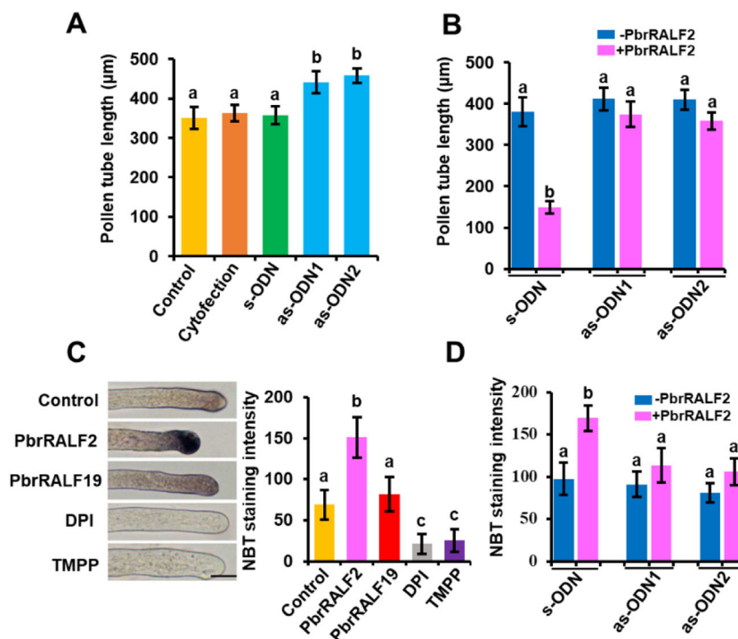
Fig. 4 PbrRALF2-induced increase in reactive oxygen species and inhibition of pollen tube growth are mediated by PbrCrRLK1L13. A Knockdown of the expression of PbrCrRLK1L13 (as-ODN) promoted pollen tube growth ( P < 0.05 , n = 3 ), whereas the s-ODN and cytofection control did not. UT indicates no treatment controls. Thirty-five pollen tubes were measured in each of three independent experiments. Different letters indicate significant differences, as determined by one-way ANOVA. B Inhibition of pollen tube growth was not sensitive to PbrRALF2 in the PbrCrRLK1L13 knockdown group compared with the significant inhibition of pollen tube growth in the s-ODN control group ( P < 0.05 , n = 4 ). Three independent experiments were conducted. Different letters indicate significant differences, as determined by two-way ANOVA. C PbrRALF2 induces reactive oxygen species (ROS) production in pollen tubes. Representative images of pollen tubes incubated with nitroblue tetrazolium (NBT) under different treatments for 30 min (left panel). Scale bar = 40 μm. Experiments were repeated at least three times with similar results. PbrRALF2 significantly increased the mean pixel intensity of the pollen tube tip ( P < 0.05 , n = 3 ; right panel), which indicated an increase in ROS, but PbrRALF19 did not. Different letters indicate significant differences, as determined by one-way ANOVA. D PbrRALF2 did not increase ROS in the as-ODN-treated PbrCrRLK1L13 pollen tube tips. Three independent experiments were conducted. Different letters indicate significant differences, as determined by two-way ANOVA
