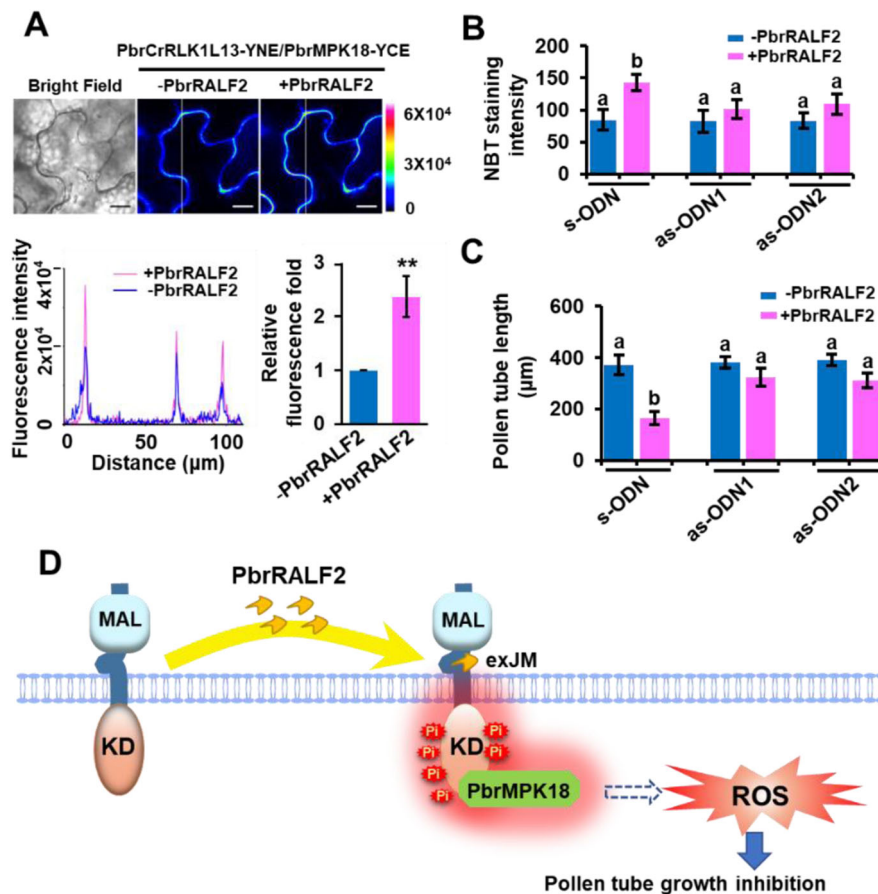
Fig. 6 PbrRALF2 enhances the PbrCrRLK1L13-PbrMPK18 interaction, and PbrMPK18 is required for PbrRALF2 signaling. A Interaction of PbrCrRLK1L13 with PbrMPK18 analyzed by BiFC in N. benthamiana epidermal cells. The interaction levels of PbrCrRLK1L13 and PbrMPK18 were significantly enhanced by 1 \mu\text{M} PbrRALF2. (** represents P < 0.01 ; Student's t test). Data points are presented as the means \pm s.e.m. Scale bar = 20 \mu\text{m} . B PbrMPK18 is required for PbrRALF2-induced ROS accumulation. PbrMPK18 was knocked down by as-ODN1 and as-ODN2, with s-ODN as a negative control. PbrRALF2 (1 \mu\text{M} ) was used to treat the pollen tubes. ROS accumulation was tested by NBT staining. Thirty-five pollen tubes were measured in each of three independent experiments. Different letters indicate significant differences, as determined by two-way ANOVA. C Inhibition of pollen tube growth was not sensitive to PbrRALF2 when PbrMPK18 was knocked down by as-ODN in pollen tubes. Thirty-five pollen tubes were measured in each of three independent experiments. Different letters indicate significant differences, as determined by two-way ANOVA. D Proposed model for PbrRALF2 perception in pollen tubes of pear. After PbrRALF2 binds to the exJM region of PbrCrRLK1L13, phosphorylation of PbrCrRLK1L13 is enhanced. Under the mediation of PbrMPK18, phosphorylated PbrCrRLK1L13 increases ROS production in pollen tubes. Excessive ROS production eventually inhibits the growth of pollen tubes
