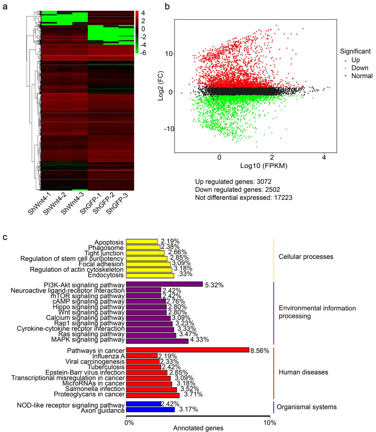
Figure 6. RNA sequence analysis of shWnt4-treated HaCaT cells. (a) Cluster analysis of the differentially expressed genes. (b) M vs A plot of the differentially expressed genes. (c) Pathway type cluster in KEGG analysis of the differentially expressed genes. n = 3 . ShWnt4 shRNA of Wnt4 mediated by lentivirus, ShGFP the empty vector for shWnt4
