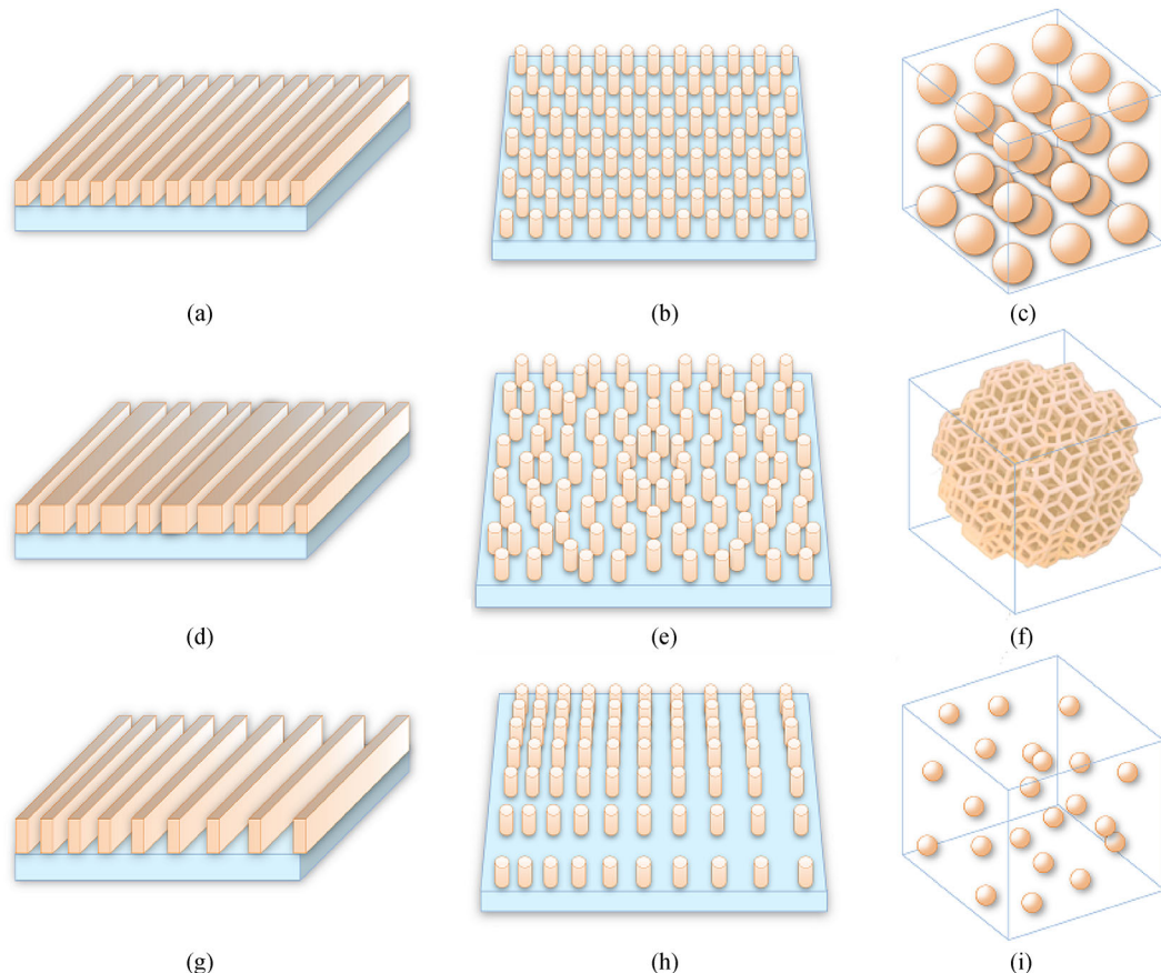
Fig. 5 Photonic crystals for DFB cavities. (a) 1D gratings; (b) 2D periodic structure; (c) 3D periodic structure; (d) Fibonacci quasi-crystals; (e) 2D quasi-crystals; (f) 3D quasi-crystals; (g) Chirped gratings; (h) 2D gradual periodic structure; (i) 3D random structure
