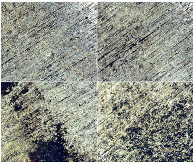
Figure 6. Corrosion at the head of copper tube. Source (s): Authors’ own work
