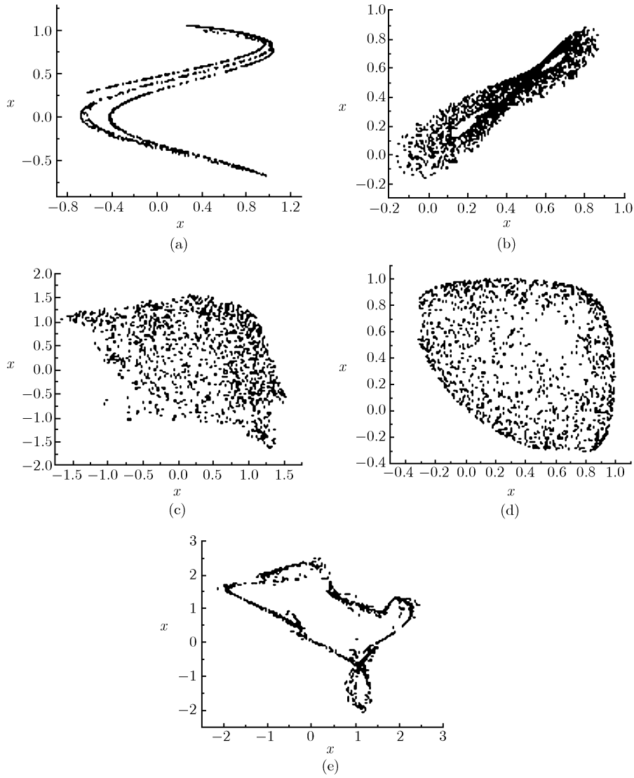
Fig. 5 (a) Chaotic attractor obtained from the map (66) with a_4 = -1.6 , a_3 = 0.1 ; (b) Chaotic attractor obtained from the map (68) with a_1 = 0.7 , a_2 = 0.85 ; (c) Chaotic attractor obtained from the map (74) with a_1 = 0.4 , a_2 = -0.4 ; (d) Chaotic attractor obtained from the map (75) with a_3 = -1 , a_7 = -1.8 ; (e) Chaotic attractor obtained from the map (76) with a_1 = 0.5 , a_9 = -0.83 .
