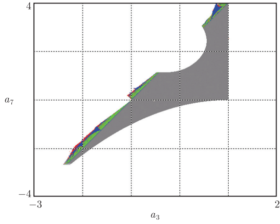
Fig. 3 Regions of dynamical behaviors in the a_3a_7 -plane for the map (75).
