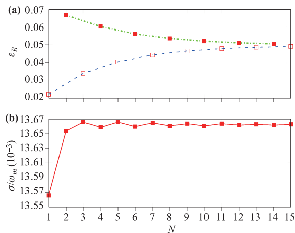
Fig. 7 The length of the cavity chain is changeable by increasing bare cavities on both side of the optomechanical cavity, and both the optomechanical interaction and the probe field are at the middle cavity. In panel (a), the value of the optomechanical transparency dip as a function of the number N of bare optical cavities in one side of the optomechanical cavity, the number is odd or even shown in blue dashed or green dashed-dotted curve, respectively; in panel (b), the red solid curve shows that the normalized frequency \sigma/\omega_m , corresponding to the transparency dip, changes over the number of bare optical cavity.
