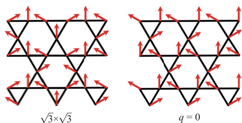
Fig. 1 Kagome lattice with the configurations of spins for the \sqrt{3} \times \sqrt{3} and q = 0 states.
