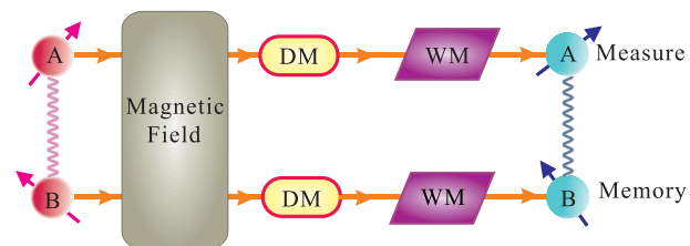
Fig. 7 The schematic diagram for the entire evolution with the time from the left to right in the current scenario. Note that, DM means Dzyaloshinskii-Moriya interaction and WM stands for quantum weak measurement.
