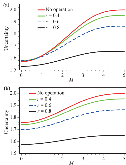
Fig. 5 Measurement uncertainty versus the magnetic field M with regard to different operational strengths r . r ranges from 0 to 0.8 from top to bottom. Here, (a) T = 3.0 and (b) T = 4.0 . For all plotted with J_x = 13/3 , J_y = -7/3 , D_x = 0.2 , J_z = 1.0 , m = 0.5 , \theta = \pi/2 and \phi = 0 .
