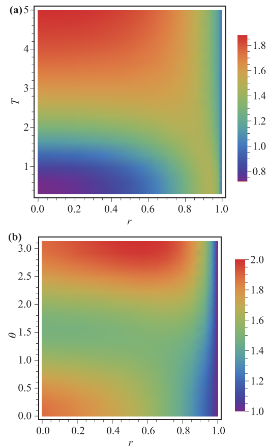
Fig. 6 (a) The dynamic of EUR with respect to T and r . The amplitude angle of the initial state \theta = \pi/2 is chosen. (b) The dynamic of EUR with respect to \theta and r . The field temperature is taken as T = 5/2 . For all plots, J_x = 13/3 , J_y = -7/3 , M = 0.5 , J_z = 1.0 , m = 0.5 and the phase \phi = 0 .
