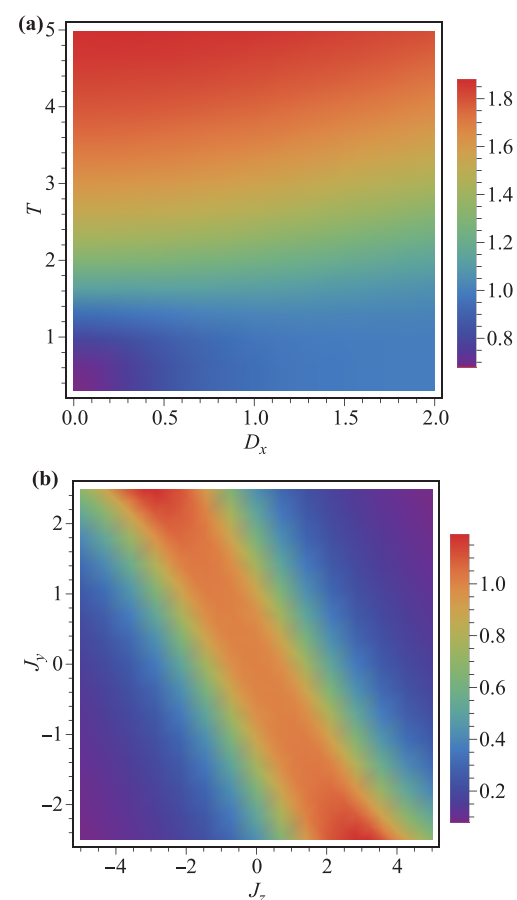
Fig. 4 (a) The dynamic of EUR with respect to T and D_x . Here, we take J_z = 1.0 and J_y = -7/3 . (b) The dynamic of EUR with respect to J_y and J_z . Here, we take T = 1.0 and D_x = 0.2 . For all plots, we take J_x = 13/3 , M = 1.0 , m = 0.5 , \theta = \pi/2 and \phi = 0 .
