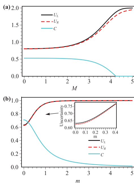
Fig. 3 Entropic uncertainty, concurrence ( C ) versus the magnetic field M and the inhomogeneity m respectively. In this figure, black solid lines depict U_L , red dash-dotted lines depict U_R and blue solid lines depict the concurrence. Noting that, U_L stands for the left item of Eq. (3) and U_R represents the right item of Eq. (3). For all, J_x = 13/3 , J_y = -7/3 , J_z = 1.0 , D_x = 0.2 , T = 1.0 , \theta = \pi/2 and \phi = 0 . Additionally, in (a) we have m = 0.5 , and M = 1.0 is chosen in (b).
