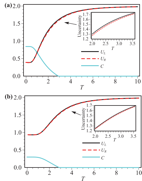
Fig. 1 Entropic uncertainty, concurrence ( C ) versus the temperature T . Noting that, U_L stands for the left-hand side of (3) and U_R represents the right-hand side of (3). In the Graphs, the black solid lines describe U_L , the red dash-dotted lines describe U_R and the blue solid lines describe the system's concurrence. (a) m = 0.2 and (b) m = 1.0 . For all plotted with J_x = 13/3 , J_y = -7/3 , J_z = 1.0 , M = 1.0 , D_x = 0.2 , \theta = \pi/2 and \phi = 0 .
