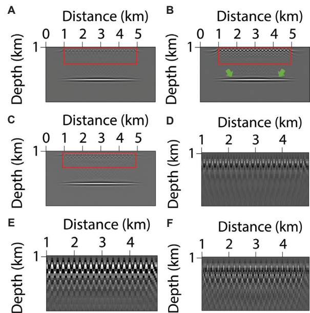
Figure 9. FWI velocity model comparison. (A) Reference solution without dispersion. (B) Result from the conventional method with artifacts. (C) Result from the proposed optimized method. (D–F) Zoomed-in views of the shallow target area corresponding to (A–C).
