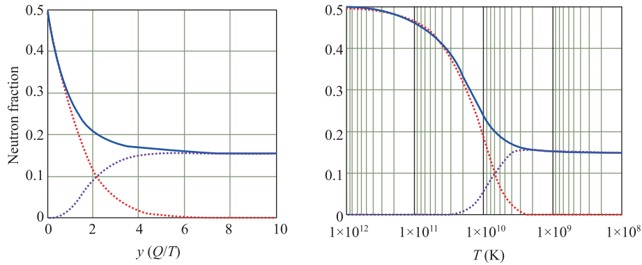
Fig. 10.2 The neutron fraction \hat{X}_n as a function y in the left panel and a function of the temperature T in the right panel. The solid curves (blue) are the neutron fraction \hat{X}_n , the dotted curves (red) are the equilibrium solution X_n^{(\text{eq})} , and the dashed curve (brown) the second term of the right-handed side of the neutron fraction solution Eq. (10.64).
