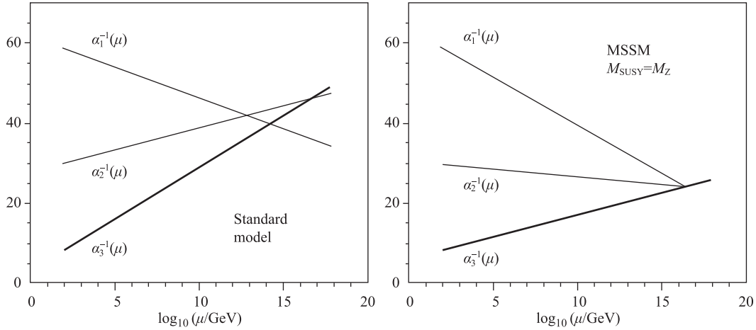
Fig. 5.1 High energy behavior of the SU(3), SU(2), and U(1) couplings constant. The left panel is for the standard model in which the couplings are not unified, while, as shown in the right panel, in the minimal supersymmetric model the couplings are unified around 10^{16} GeV. These figures are from Ref. [99] but rearranged.
