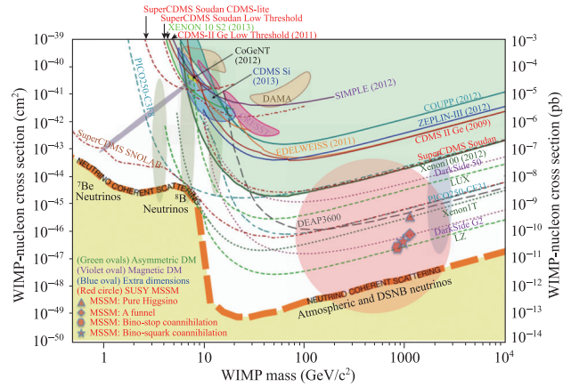
Fig. 8.15 Figure and its caption are from Ref. [205]. The solid curves are the established limits, and the dotted/dashed curves are the planned ones as of the end of 2013. The LUX bound represented by the green dashed curve is now an established bound which is the strongest for WIMP mass greater than 8 GeV.
