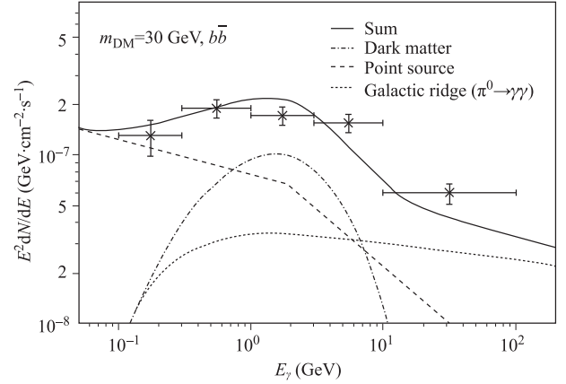
Fig. 8.8 The figure is adopted from [183]. The result of a 30 GeV dark matter particle annihilates into the b\bar{b} channel with an annihilation cross section is v\sigma \sim 6 \times 10^{-27} \text{ cm}^3/\text{s} .
