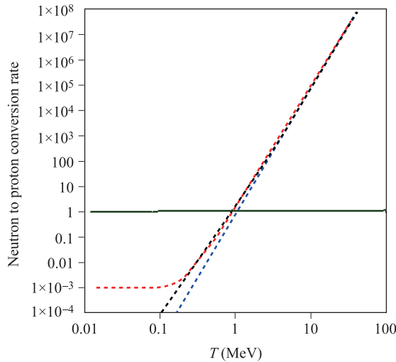
Fig. 10.1 The neutron to proton rate \lambda(n \rightarrow p) . The horizontal axis is the temperature in units of MeV ( 1 \text{ MeV} = 1.1605 \times 10^{10} \text{ K} ). The various curves are, the dotted (red) curve: the Weinberg exact expression given in Eq. (10.35), the dashed curve (blue): The high temperature approximation given in Eq. (10.41); the dash-dotted (black) curve: The BBF approximate expression without the neutron decay contribution as given in (10.34); The solid (dark green, almost horizontal) curve: The ratio of the BBF full approximation given in Eq. (10.32) to the Weinberg expression Eq. (10.35).
