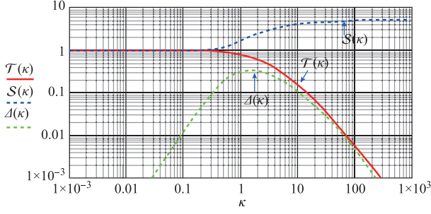
Fig. 12.8 Transfer functions defined in Eq. (12.226).
