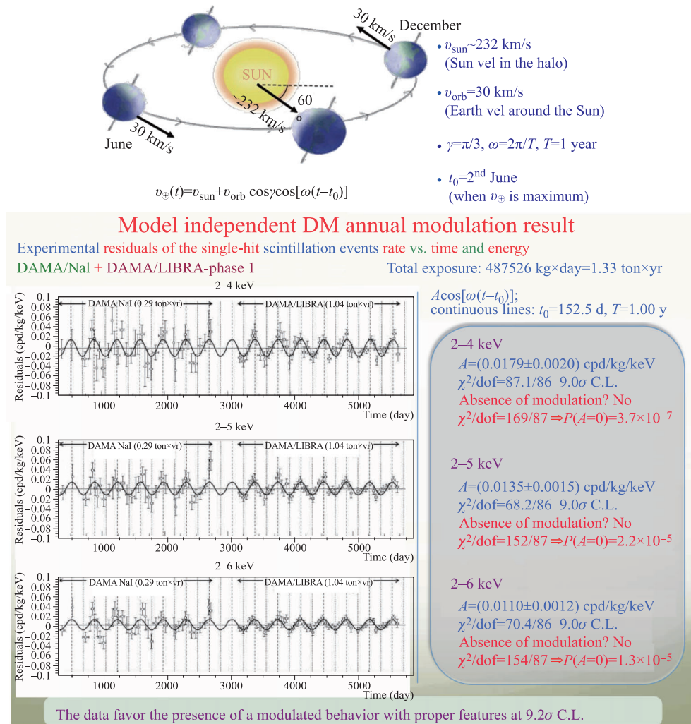
Fig. 8.1 Upper: The velocity modulation of an Earth laboratory. Lower: The DAMA/LIBRA and DAMA/NaI annual modulation data and analysis. The plots are adopted from [145] and [146], which together with other presentations made on DAMA can be found in Downloads of the collaboration homepage [147].
