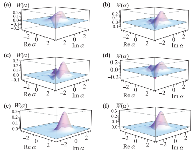
Fig. 1 Wigner distribution of the photon-modulated state (ta + ra^\dagger)^m |\gamma\rangle ( r^2 + t^2 = 1 ) for different parameters m, r and \gamma , where the values of (m, r, \gamma) are respectively (a) (1, 0.5, 0.2), (b) (3, 0.5, 0.2), (c) (4, 0.5, 0.2), (d) (3, 0.5, 0.1), (e) (3, 0.5, 0.5), (f) (3, 0.2, 0.2).
