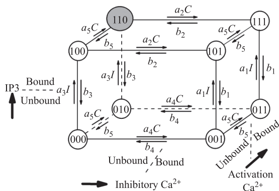
Fig. 1 Schematic diagram of the state transitions for the DYK IP 3 R subunit. C and I represent the concentrations of Ca 2+ and IP 3 in the cytoplasm, respectively
