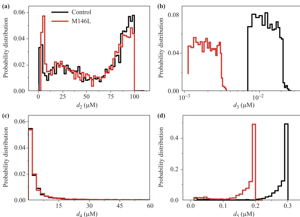
Fig. 4 Comparison of the probability distributions of dissociation constants d_i between the control and M146L cells. (a–d) show the parameter distributions of d_2 , d_3 , d_4 , and d_5 , respectively. The black lines represent the control cells and the red lines represent the M146L cells.
