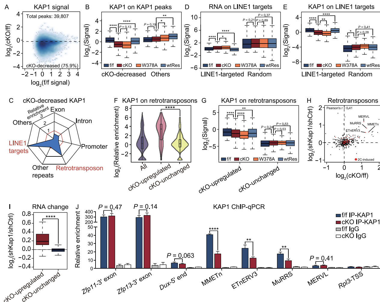
Figure 4. YTHDC1 facilitates the genome recruitment of KAP1 in ESCs. (A) Scatter plot showing the KAP1 ChIP signal in Ythdc1 f/f ESCs (x-axis) and fold change of the signal upon Ythdc1 depletion in ESCs (y-axis) on 39807 KAP1 peaks identified in f/f ESCs. A total of 30217 Ythdc1 cKO-decreased KAP1 peaks were defined as KAP1 peaks with \log_2(\text{fold change}) < -0.2 . (B) KAP1 ChIP signal was significantly decreased on Ythdc1 cKO-decreased KAP1 peaks (defined in (A)) in Ythdc1 cKO and W378A ESCs. (C) Ythdc1 cKO-decreased KAP1 peaks (defined in (A)) were enriched at LINE1 RNA-targeted loci (Lu et al., 2020) and retrotransposons in genome. (D and E) RNA level was upregulated and KAP1 ChIP signal was decreased at LINE1 RNA-targeted loci (24202 regions defined by Lu et al., 2020) in Ythdc1 cKO and W378A ESCs. An equal number of random loci serve as the control. (F) Violin plot showing that Ythdc1 cKO-decreased KAP1 peaks (defined in (A)) were more enriched on Ythdc1 cKO-upregulated retrotransposons compared to Ythdc1 cKO-unchanged retrotransposons in ESCs. Ythdc1 cKO-upregulated/unchanged retrotransposons were defined as in Fig. 3F. (G) KAP1 ChIP signal was significantly decreased on Ythdc1 cKO-upregulated retrotransposons (defined as in Fig. 3F) in Ythdc1 cKO and W378A ESCs. (H) Scatter plot showing fold change of the retrotransposon level upon Ythdc1 depletion (x-axis) or Kap1 KD (y-axis) in ESCs. Representative 2C-related retrotransposons consistently upregulated in Ythdc1 cKO ESCs and Kap1 KD ESCs are labeled in the plot. Pearson's correlation coefficient was calculated in R. shCtrl, control shRNA expressed. shKap1, Kap1 shRNA expressed. (I) Ythdc1 cKO-upregulated retrotransposons were significantly more derepressed compared to Ythdc1 cKO-unchanged retrotransposons upon Kap1 KD in ESCs. Ythdc1 cKO-upregulated/unchanged retrotransposons were defined as in Fig. 3F. (J) KAP1 ChIP-qPCR analysis showing the unaffected KAP1 binding at 5' end of Dux locus, 3' exons of Zfp11/Zfp13 genes and MERVL elements, and the significantly decreased KAP1 binding at certain 2C-related retrotransposons upon Ythdc1 depletion in ESCs. TSS of Rpl3 gene which is not targeted by KAP1 serves as a negative control. Relative enrichment was calculated as the percent of input normalized to enrichment at the negative control intergenic chromosome 11 (int-chr11). Two independent reactions for each IP were performed. Data are presented as means with SDs ( n = 3 technical replicates). Means of replicates were used to generate the summarized data in (A, B, D, E and G–I). Significance (* P < 0.05 , ** P < 0.01 , **** P < 0.0001 ) was calculated with two-tailed Student's t test (paired in (B, D, E and G) and unpaired in (F, I and J)). See also Fig. S5.
