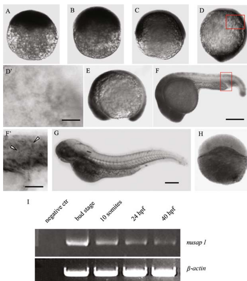
Figure 3. Expression profile of nusap1 in zebrafish. nusap1 transcripts were probed using in situ hybridization at the following stages: (A) One cell stage; (B) 30% epiboly stage; (C) 50% epiboly stage; (D) Bud stage; (E) 10 somites stage; (F) 24 hpf (scale bar indicates 0.5 mm in panels A–D, E, F and H); (G) 3 dpf (scale bar indicates 0.5 mm). Panels D' and F' were inserts from D and F, respectively. Scale bars indicated 100 \mu m. (H) Control assay using sense-RNA probe in parallel, and 30% epiboly embryo was listed as example. Embryos in panels E–G display a lateral view with anterior to left orientation; the others display a lateral view with animal pole to upward orientation.
