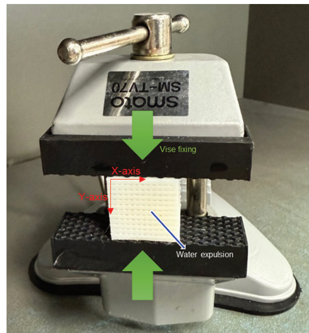
Figure 7. Preventing deformation of permafrost simulation models due to volume expansion
