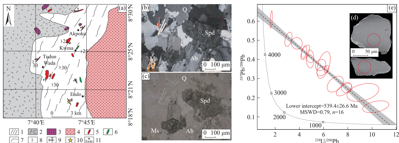
Fig. 1. a–Simplified geologic map of Nasarawa area; b–Perpendicular polarized light photomicrograph of pegmatite; c–plane polarized light photomicrograph of pegmatite; d–CL images of cassiterite; e–U–Pb concordia diagram for cassiterites from Nasarawa lithium deposit. 1–mica schist; 2–orthogneiss; 3–Pan-African granite; 4–Mesozoic granite complexes; 5–pegmatitic dyke; 6–basic dyke; 7–geological boundary; 8–foliation and occurrence; 9–rare-metal deposit; 10–sampling point; 11–village name. Spd–spodumene; Ab–albite; Q–quartz; Ms–muscovite.
