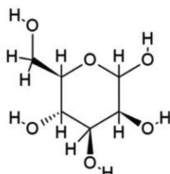
D-Mannose( C_6H_{12}O_6 ) MW: 180.16 g/mol
