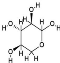
D-Xylose( C_5H_{10}O_5 ) MW: 150.13 g/mol
