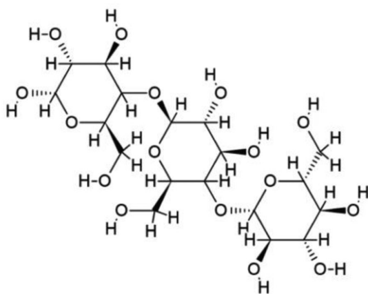
Beta-Glucan( C_{18}H_{32}O_{16} ) MW: 504.4 g/mol
