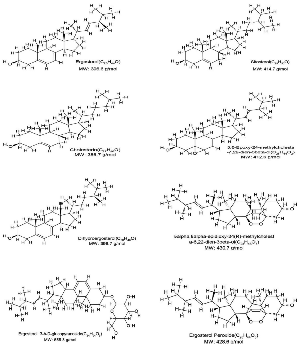
Figure 5. Molecular structural formulae of the primary sterols in Ophiocordyceps sinensis .
