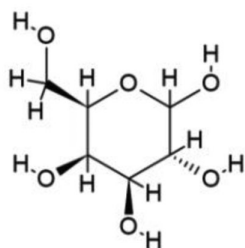
D-Galactose( C_6H_{12}O_6 ) MW: 180.16 g/mol
