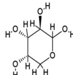
L-Arabinose( C_5H_{10}O_5 ) MW: 150.13 g/mol
