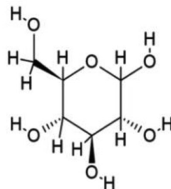
D-Glucose( C_6H_{12}O_6 ) MW: 180.16 g/mol
