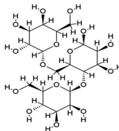
D-Galacto-d-mannan( C_{18}H_{32}O_{16} ) MW: 504.4 g/mol
