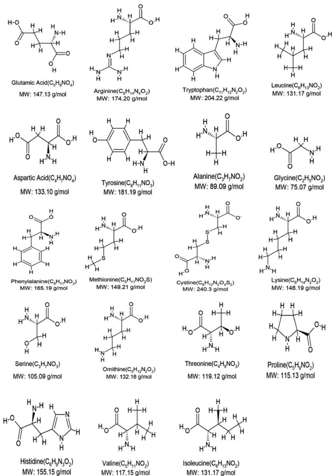
Figure 6. Molecular structural formulae of the principal amino acids in Ophiocordyceps sinensis .
