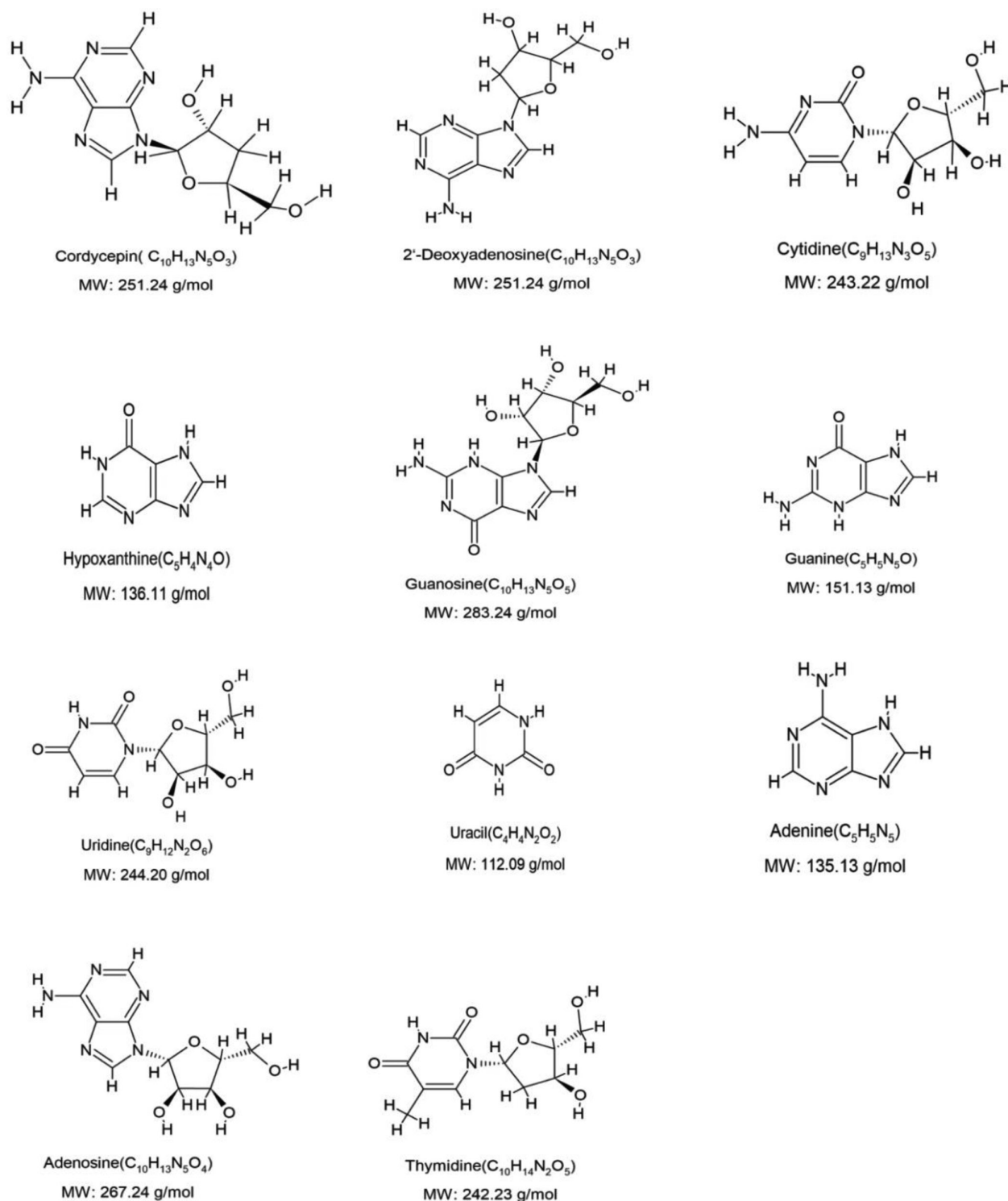
Figure 3. Molecular structural formulae of the principal nucleosides in Ophiocordyceps sinensis .
