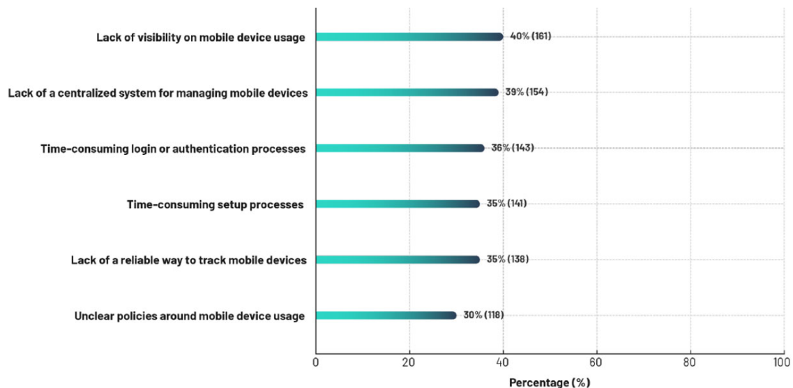
Figure 2. Shared-use mobile device management challenges for the information technology department
