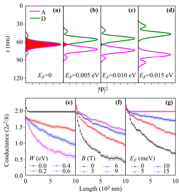
Fig. 4 (a–d) Corresponding wavefunction distributions of the kink states in valleys K and K' (modes A and D, respectively, labeled in Fig. 1(c)) at different Fermi energies E_F = 0 (a), 0.005 (b), 0.010 (c), and 0.015 eV (d) but the same magnetic field strength B = 9 T. (e, f) Average conductance vs. device length under different parameter strengths. In (e), the Fermi level is E_F = 0.01 eV, there is no magnetic field, and the disorder strength is varied as W = 0, 0.2, 0.4 , and 0.6 eV. The band gap is set as 2U = 0.04 eV. In (f), the Fermi level is E_F = 0.006 eV, the magnetic field strength is varied as B = 0, 3, 6 , and 9 T, and the disorder strength is W = 0.6 eV. In (g), the magnetic field strength is B = 9 T, the Fermi level is varied as E_F = 0, 5, 10 , and 15 meV, and the disorder strength is W = 0.06 eV. Each point is an average of 30 samples with different disorder configurations.
