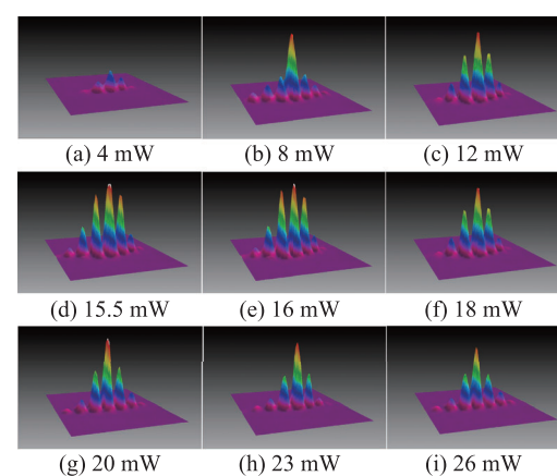
Fig. 5 The three-dimensional output diffraction patterns with different coupling laser powers.
