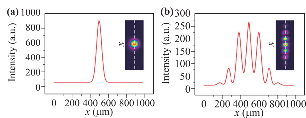
Fig. 2 The spatial intensity distribution of probe beam through the vapor cell without (a)/with (b) the standing-wave field. The line is the intensity distribution of the section profile of the output pattern versus x axis. The inset is the direct output profile of the probe beam from the CCD, and the dotted line notifies the position of the section.
