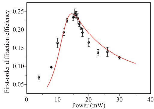
Fig. 6 The first-order diffraction efficiency of electromagnetically induced grating with different coupling laser powers. The red line is the theoretical simulation and dots are experimental results.
