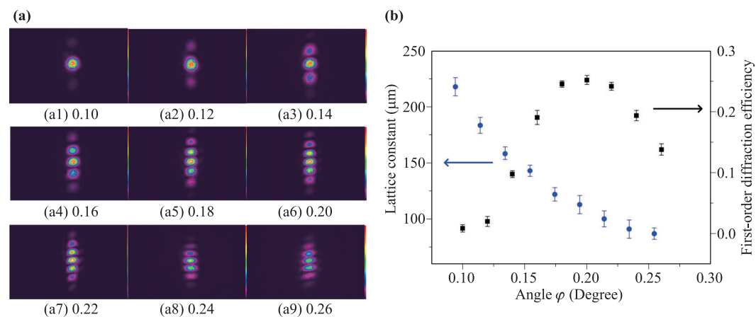
Fig. 3 (a) The diffraction patterns with different angles \varphi (in degree) of two coupling lasers. (b) The grating constant (circles) and the first-order diffraction efficiency (squares) as a function of the angle \varphi .
