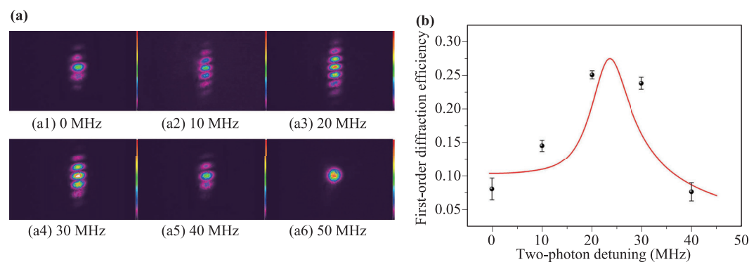
Fig. 4 (a) The output diffraction patterns with different two-photon detunings. (b) The corresponding first-order diffraction efficiency with different two-photon frequency detunings. The red line is the theoretical fitting and dots are experimental results.
