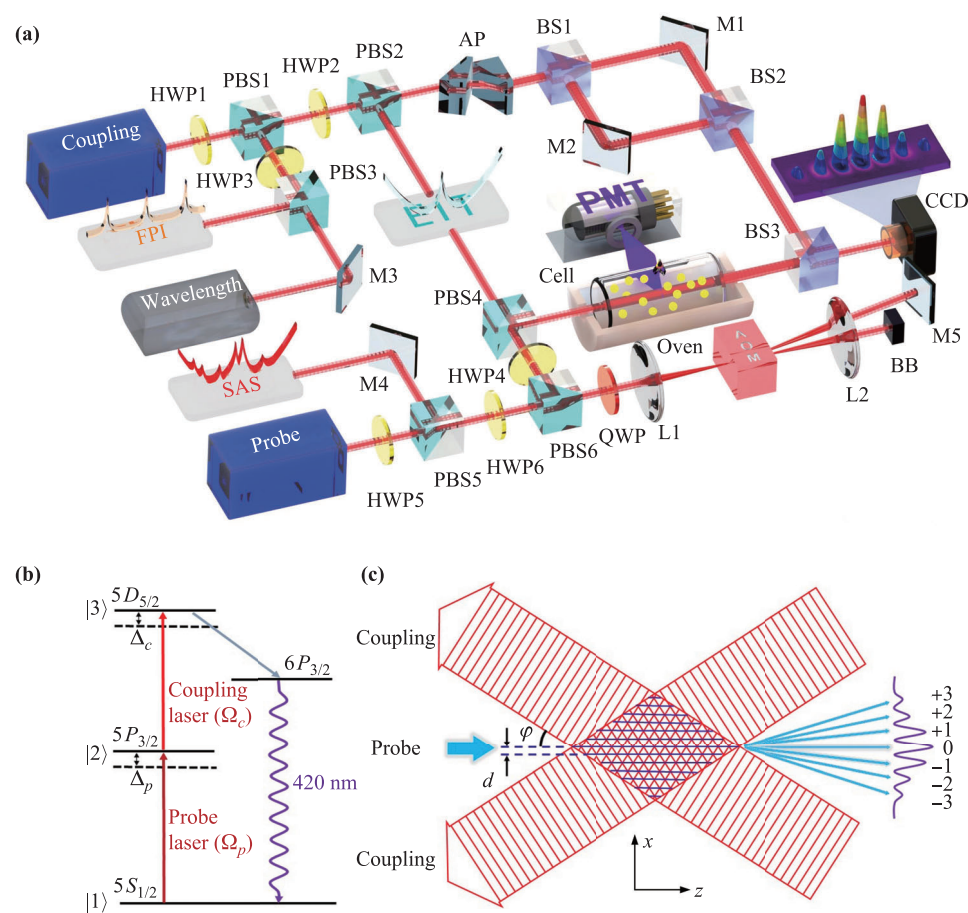
Fig. 1 (a) Experiment setup, HWP: Half-wave plate, PBS: Polarization beam splitter, AP: Anamorphic prism, BS: Beam splitter, M: High reflection mirror, FPI: Fabry–Perot interferometer, EIT: Electromagnetically induced transparency, PMT: photomultiplier tube, SAS: Saturation absorption spectroscopy, CCD: Charge-coupled device, QWP: Quarter-wave plate, L: Lens, AOM: Acousto-optic modulator, BB: Beam block. (b) Schematic diagram of a cascade-type coherent rubidium system. (c) Illustration of electromagnetically induced grating by a standing-wave ( x direction) coupling field and a traveling wave ( z direction) probe field.
