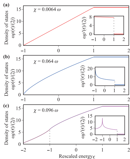
Fig. 5 The density of states \rho(\epsilon) , in units of 2j/\omega , versus the rescaled energy \epsilon when mode a is in coherent state |\alpha\rangle_a . The inserted panels plot the first derivative of the density of states.
