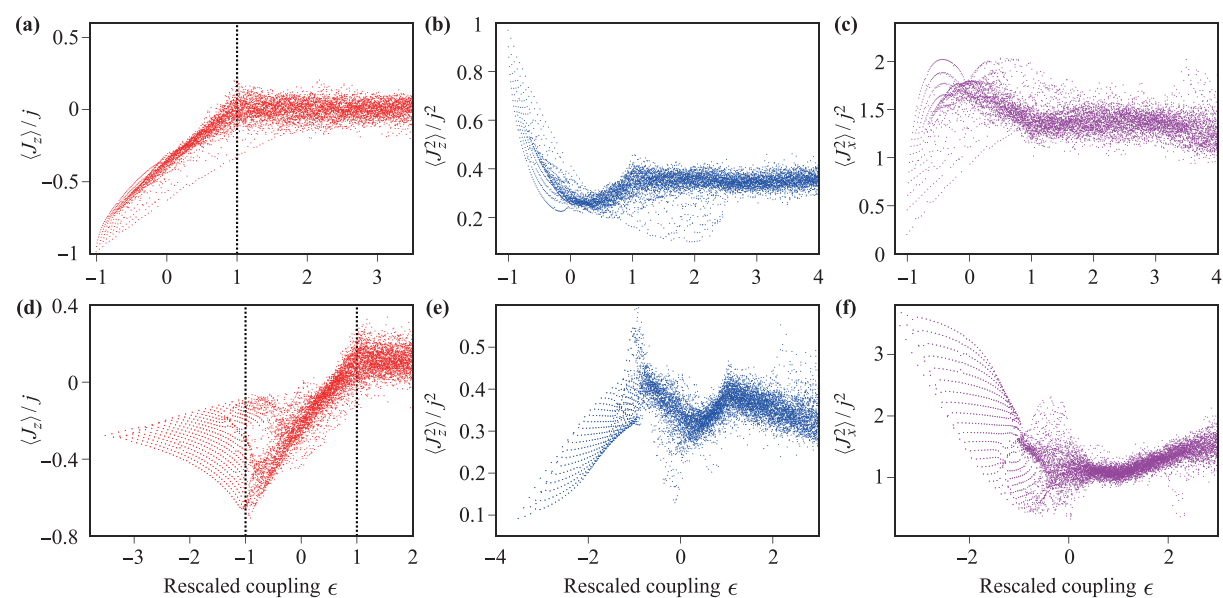
Fig. 6 Peres lattice of the proposed model using the Peres operators J_z (left panel), J_z^2 (middle panel) and J_x^2 (right panel) by considering a to be in |0\rangle_a (upper row) and |\alpha\rangle_a (bottom row). We use j = 30 and truncate N_b^{\max} = 200 , \Omega = \omega = 1 , g_0 = 2.49 \times 10^{-5}\omega , and \chi = 0.99\omega .
