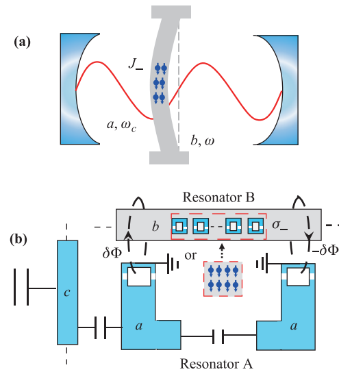
Fig. 1 The schematic diagram of the proposed system. (a) A schematic illustration of the proposed model in a quadratically-coupled optomechanical system. An ensemble of two-level atoms is embedded in a membrane (with bosonic mode b ) with atom-field coupling strength \lambda , which describes the normal Dicke model. The single bosonic mode b interacts with an ancillary mode a with a quadratic coupling g_0 , which can be realized by placing the membrane in the node of the cavity mode a . The mode a is prepared in a coherent state |\alpha\rangle_a . (b) A proposed implementation of the proposed system in a superconducting circuit with the ability of simulating a quadratic optomechanical coupling [45].
