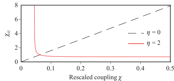
Fig. 2 The effective rescaled coupling strength \chi_\alpha with respect to \chi . We consider the ancillary mode is in coherent state |\alpha\rangle_a . \eta = 0, g_0 = 2.49 \times 10^{-5}\omega for black-dashed curve and \eta = 2, g_0 = 2.51 \times 10^{-5}\omega for red-solid curve. Other parameters are \omega = \Omega = 1 , and |\alpha|^2 = 10^4 .
