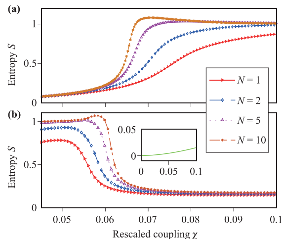
Fig. 3 The von Neumann entropy S corresponds to the rescaled coupling \chi for different numbers of atoms N . Ancillary mode a is prepared in |\alpha\rangle_a for the main panel and vacuum state |0\rangle_a for the inserted panel. \Omega = \omega = 1 , |\alpha|^2 = 10^4 for both, (a) \eta = 0 and g_0 = 2.49 \times 10^{-5}\omega and (b) \eta = 2 , g_0 = 2.51 \times 10^{-5}\omega are considered, respectively.
