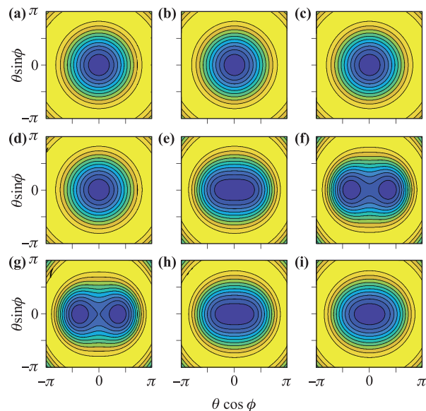
Fig. 4 Contourf of the energy surface \epsilon versus \theta and \phi [see Eq. (20)]. In the top row, \eta = 0 and ancillary mode is prepared in vacuum state |0\rangle_a . From the left to right, the rescaled couplings are 0.01\omega, 0.064\omega, 0.096\omega . The middle row shows the results considering \eta = 0 , ancillary mode a in coherent state |\alpha\rangle_a . The rescaled couplings are same as the top row. The bottom shows \eta = 2 , ancillary mode being in |\alpha\rangle_a . The parameters from left to right are \chi = 0.05\omega, 0.064\omega, 0.096\omega , respectively. Here \chi_{ac} = 2\lambda_\alpha/\sqrt{\Omega\omega_\alpha} , g_0 = 2.49 \times 10^{-5}\omega for \eta = 0 and g_0 = 2.51 \times 10^{-5}\omega for \eta = 2 are considered.
