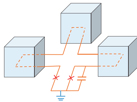
Fig. 3 Setup for three 3D microwave cavities inductively coupled to a transmon qutrit. Electronic circuit of a transmon qutrit consists of two Josephson junctions and a capacitor.
