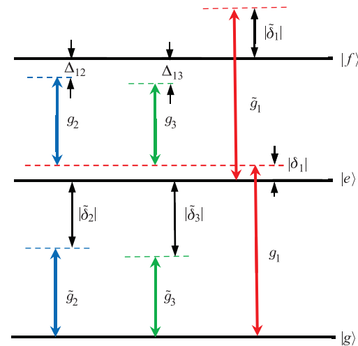
Fig. 4 Illustration of the unwanted coupling between cavity 1 and the |e\rangle \leftrightarrow |f\rangle transition of the qutrit (with coupling strength \tilde{g}_1 and detuning |\tilde{\delta}_1| ) as well as the unwanted coupling between cavity l and the |g\rangle \leftrightarrow |e\rangle transition of the qutrit (with coupling strength \tilde{g}_l and detuning |\tilde{\delta}_l| ) ( l = 2, 3 ). Here, |\tilde{\delta}_1| = \omega_{c_1} - \omega_{fe} and |\tilde{\delta}_l| = \omega_{eg} - \omega_{c_l} ( l = 2, 3 ). Other couplings depicted in the figure are needed, as described by the Hamiltonian (2) with n = 3 . Note that the coupling of each cavity with the |g\rangle \leftrightarrow |f\rangle transition of the qutrit is negligible because of the forbidden or very weak |g\rangle \leftrightarrow |f\rangle transition [50, 51].
