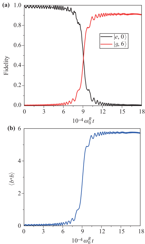
Fig. 5 (a) Fidelity of the |e, 0\rangle and |g, 6\rangle states as a function of gt with the initial state |e, 0\rangle . (b) Expectation value of the photon number \langle b^\dagger b \rangle . All results are plotted as functions of \omega_0^R t with g = 0.06\omega_0^R , v_c = 10^{-6}\omega_0^{R2} , \omega^R = 0.168\omega_0^R , and \Gamma = \gamma_m = 0.0005g .
