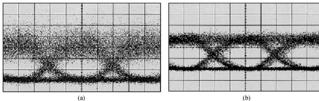
Fig. 4 Eye diagrams for spectrum noise suppress. (a) Without SOA; (b) with SOA
