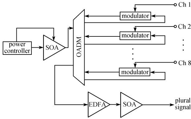
Fig. 1 WDM multiple-wavelength modulated transmitter architecture
