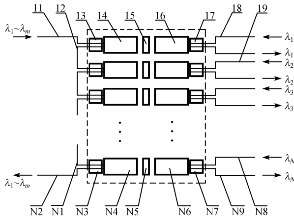
Fig. 2 Configuration of proposed OADM (11,12-N1,N2: input fibers; 13-N3: dual-fiber contact pins; 14-N4: coupling GRIN lenses; 15-N5: dense wavelength-division multiplexing (DWDM) filters; 16-N6: coupling GRIN lenses; 17-N7: dual-fiber contact pins; 18,19-N8,N9: output fibers)
