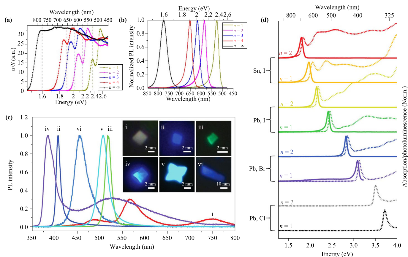
Fig. 2 (a, b) The absorption and photoluminescence spectra of BA 2 MA n-1 Pb n I 3n+1 ( n = 1-4 , 3D). Reproduced with permission from Ref. [37], Copyright © 2016 American Chemical Society. (c) Solution phase PL spectra and optical PL images (insets) of 2D perovskite nanoplates of BA 2 PbCl 4 (i), BA 2 PbBr 4 (ii), BA 2 PbI 4 (iii), BA 2 PbCl 2 Br 2 (iv), BA 2 PbBr 2 I 2 (v), and BA 2 MAPb 2 Br 7 (vi). Reproduced with permission from Ref. [42], Copyright © 2015 American Association for the Advancement of Science. (d) Solution phase absorption and photoluminescence spectra of L 2 [ABX 3 ] n-1 BX 4 , where L is an organic ligand (octylammonium, butylammonium). Reproduced with permission from Ref. [45], Copyright © 2016 American Chemical Society.
