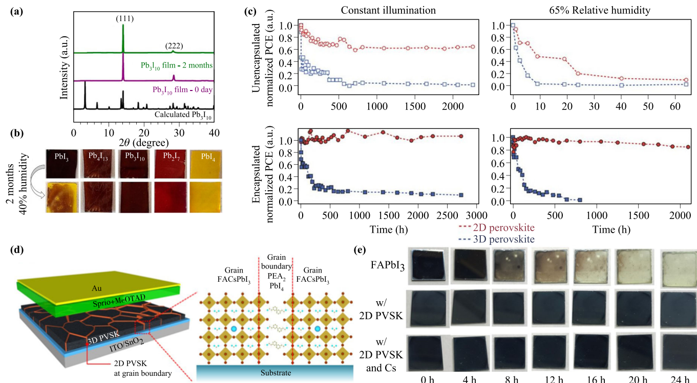
Fig. 5 (a, b) XRD patterns and photos showing the improved stability against moisture of \text{BA}_2\text{MA}_{n-1}\text{Pb}_n\text{I}_{3n+1} ( n = 1-4 ) compared with \text{MAPbI}_3 . Reproduced with permission from Ref. [36], Copyright © 2015 American Chemical Society. (c) Improved device stability of RP perovskite solar cells based on \text{BA}_2\text{MA}_3\text{Pb}_4\text{I}_{13} compared with 3D perovskite solar cells based on \text{MAPbI}_3 . Reproduced with permission from Ref. [48], Copyright © 2016 Springer Nature. (d) Scheme of \text{FAPbI}_3 passivated by \text{PEA}_2\text{PbI}_4 . (e) Improved phase stability of \text{FAPbI}_3 with passivation of \text{PEA}_2\text{PbI}_4 . d, e were reproduced with permission from Ref. [114], Copyright © 2018 Springer Nature.
