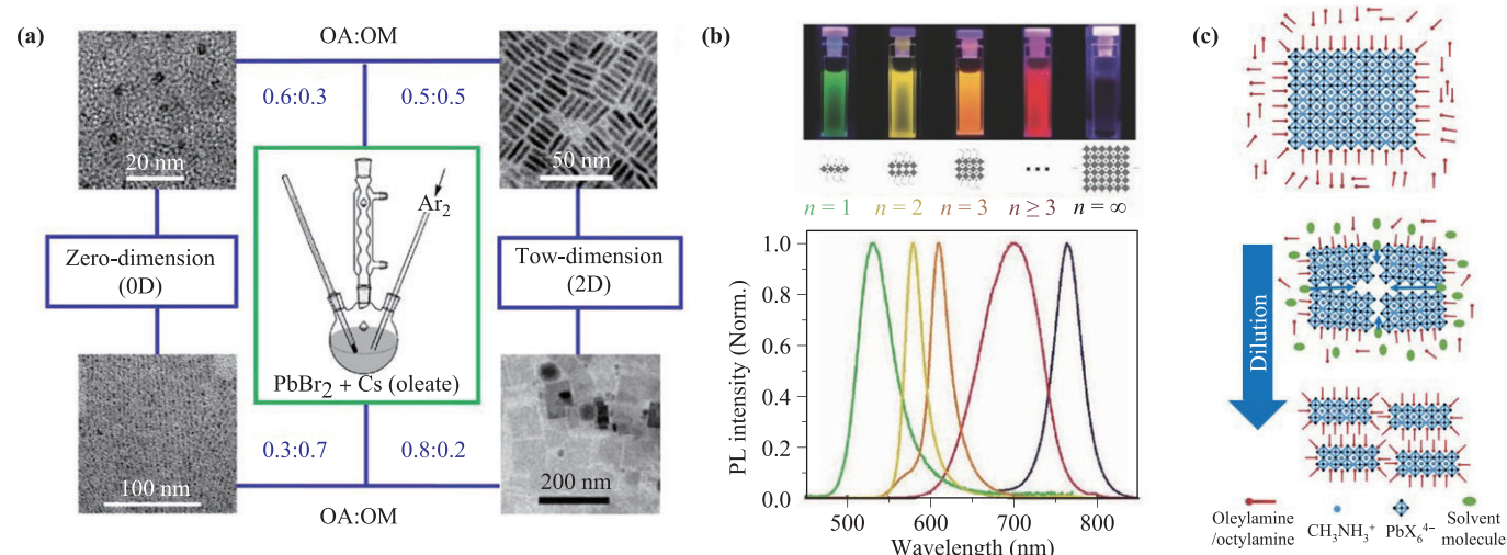
Fig. 6 (a) CsPbBr 3 NCs with various shapes by LARP method with different ratio of OA and OM. Reproduced with permission from Ref. [141], Copyright © 2016 American Chemical Society. (b) MAPbI 3 nanoplates prepared by diluting large MAPbI 3 microcrystals solution in toluene with octylamine. Reproduced with permission from Ref. [144], Copyright © 2016 John Wiley and Sons. (c) Schematic of the dilution-induced fragmentation of perovskite microcrystals into nanoplates. Reproduced with permission from Ref. [145], Copyright © 2016 American Chemical Society.
