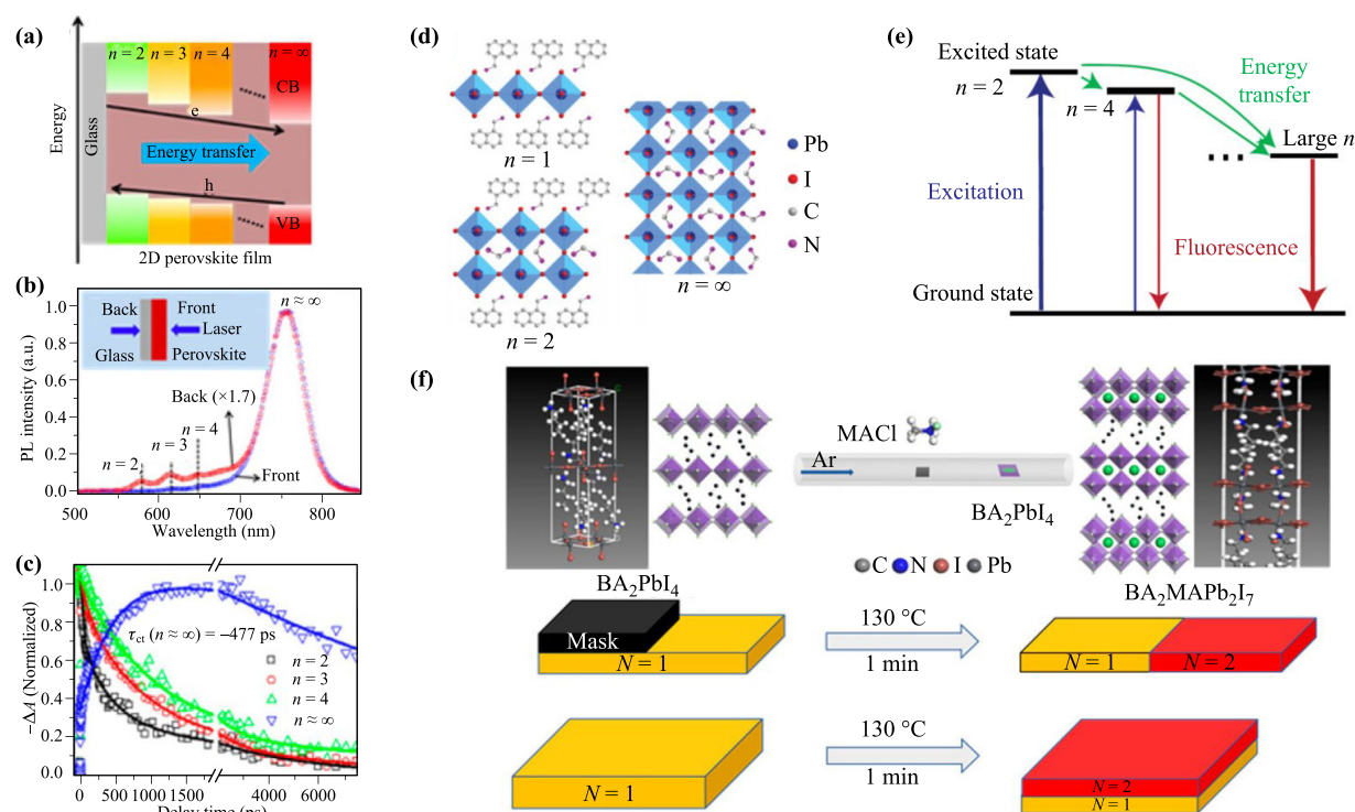
Fig. 4 (a) Comparative bandgap energy alignment of \text{BA}_2\text{MA}_{n-1}\text{Pb}_n\text{I}_{3n+1} perovskites with different n values and three possible carrier transfer mechanisms: electron and energy transfers from small- n to large- n perovskites and hole transfer from large- n to small- n perovskites. (b) PL spectra of \text{BA}_2\text{MA}_3\text{Pb}_4\text{I}_{13} perovskite film by hot-casting method illuminated from the front and back sides by a 405 nm laser. (c) Femtosecond transient absorption (TA) kinetics probed at n = 2, 3, 4 and n \approx \infty bands under back-excitation. a, b and c were reproduced with permission from Ref. [79], Copyright © 2017 American Chemical Society. (d, e) Scheme of \text{NMA}_2\text{MA}_{n-1}\text{Pb}_n\text{I}_{3n+1} (NMA: 1-naphthylmethylamine) and cascade energy transfer from smaller- n quantum wells (QWs) to larger- n QWs. d, e were reproduced with permission from Ref. [82], Copyright © 2016 Springer Nature. (f) Scheme of the gas-solid phase intercalation process to synthesize the lateral and vertical heterostructures with \text{BA}_2\text{PbI}_4/\text{BA}_2\text{MAPb}_2\text{I}_7 . Reproduced with permission from Ref. [86], Copyright © 2017 American Chemical Society.
