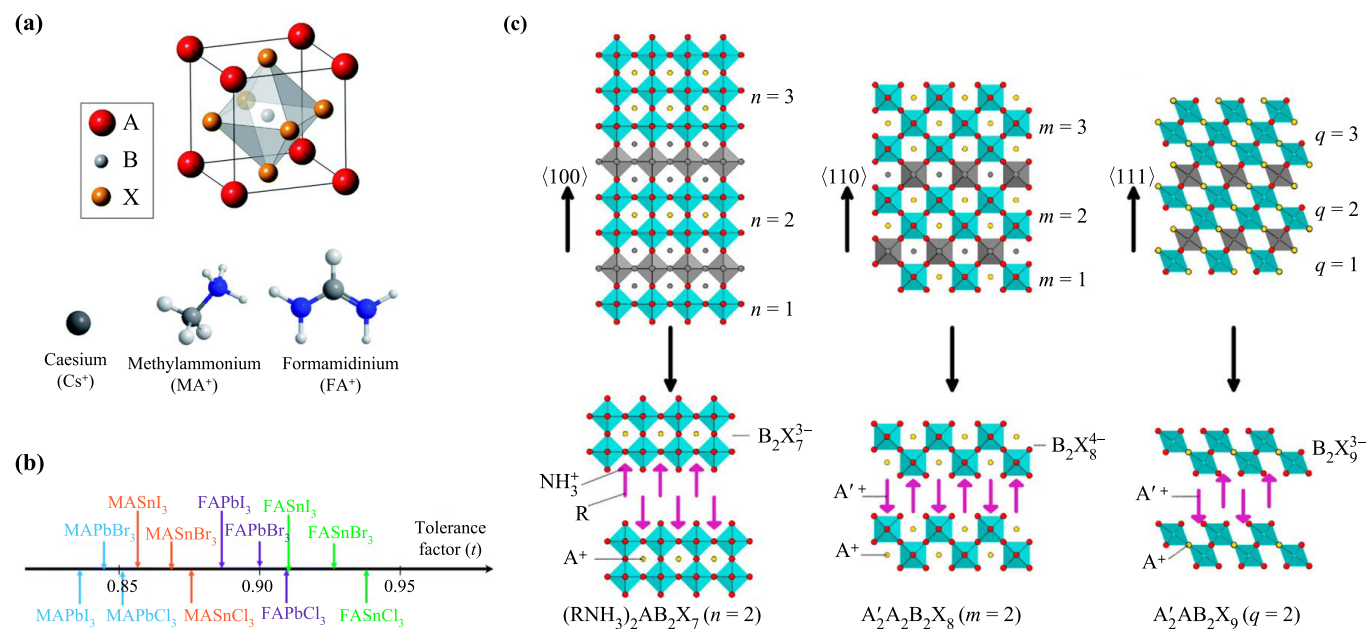
Fig. 1 (a) The crystal structure of 3D perovskite ABX_3 , with A cation of caesium ( Cs^+ ), methylammonium ( MA^+ ), or formamidinium ( FA^+ ). Reproduced with permission from Ref. [8], Copyright © 2014 The Royal Society of Chemistry. (b) Tolerance factors ( t ) of a series of 3D halide perovskites. Reproduced with permission from Ref. [9], Copyright © 2015 The Royal Society of Chemistry. (c) The structure derivation of layered 2D perovskite with long cation cutting the 3D perovskite from (100), (110) and (111) plane, respectively. Reproduced with permission from Ref. [12], Copyright © 2016 American Chemical Society.
