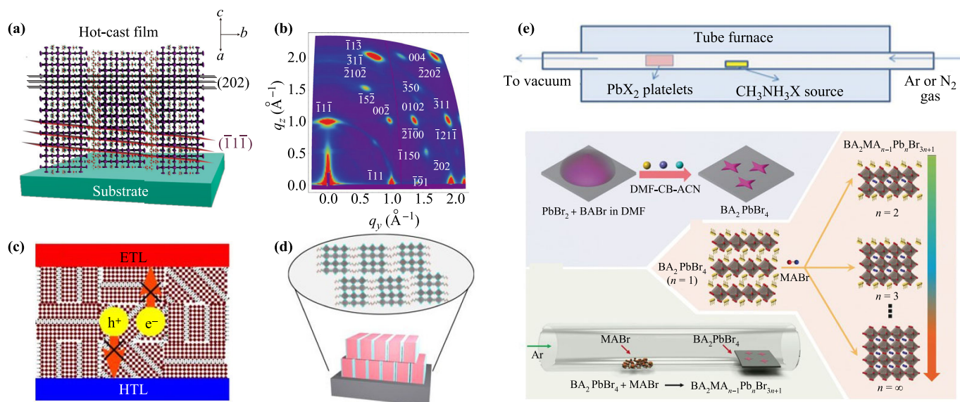
Fig. 3 (a, b) Scheme of orientation and grazing-incidence wide-angle X-ray scattering (GIWAXS) patterns for \text{BA}_2\text{MA}_3\text{Pb}_4\text{I}_{13} perovskite film by hot-casting method. Reproduced with permission from Ref. [48], Copyright © 2016 Springer Nature. (c) Scheme of disordered orientation of \text{BA}_2\text{MA}_3\text{Pb}_4\text{I}_{13} perovskite film prepared by room-temperature casting method. Reproduced with permission from Ref. [49], Copyright © 2018 Springer Nature. (d) Scheme of vertically packed quantum wells with misalignment in molecular structures. Reproduced with permission from Ref. [50], Copyright © 2018 Springer Nature. (e) Schematic of the synthesis setup for converting \text{PbX}_2 platelets by MAX vapor. Reproduced with permission from Ref. [73], Copyright © 2014 John Wiley and Sons. (f) Scheme of synthesis of \text{BA}_2\text{PbBr}_4 perovskites via a ternary solvent method and transformation of \text{BA}_2\text{PbBr}_4 into \text{BA}_2\text{MA}_{n-1}\text{Pb}_n\text{Br}_{3n+1} perovskites via chemical vapor deposition of MABr. Reproduced with permission from Ref. [78], Copyright © 2017 John Wiley and Sons.
