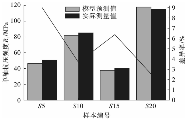
图 7 单轴抗压强度预测值与试验值对比图 Fig. 7 Comparison of predicted and tested uniaxial compressive strength values
