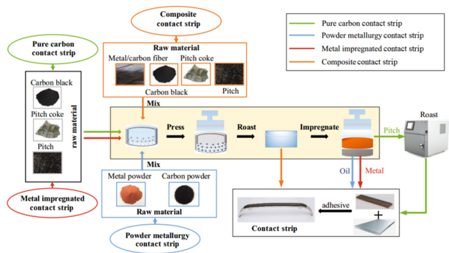
Figure 3. Schematic of the CS manufacturing process. Source(s): Wu et al. (2022a)
