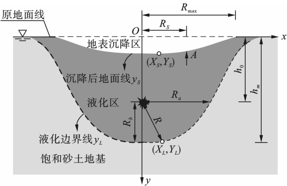
图 2 典型液化和地表沉降区示意图(单药包爆破) Fig. 2 Typical liquefaction and surface settlement area morphology( Single charge blasting)
