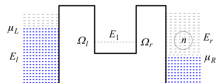
Fig. 1 Resonant tunneling through a single-level dot (see text), n denoted number of electrons arriving the right reservoir at time t .
