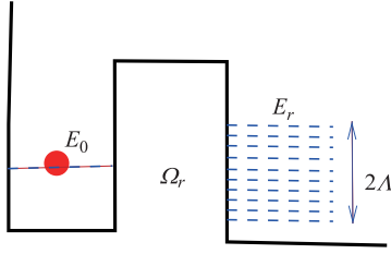
Fig. 14 Tunneling of a particle to continuum from a localized state inside the well to a reservoir of a finite bandwidth \Lambda .
