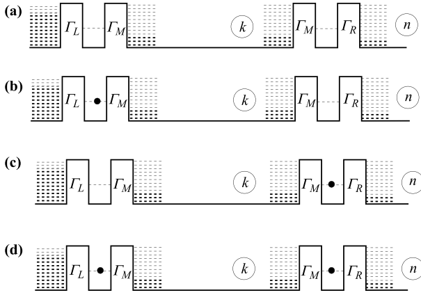
Fig. 6 Electron states of the two separated dot structure, shown in Fig. 5. \Gamma_{L,R} , \Gamma_M and \bar{\Gamma}_M are the tunneling rates between the dots and the reservoirs, and between the dots and the ballistic channel. The indices k and n denote the number of electrons penetrating to the ballistic channel and to the collector at time t .
