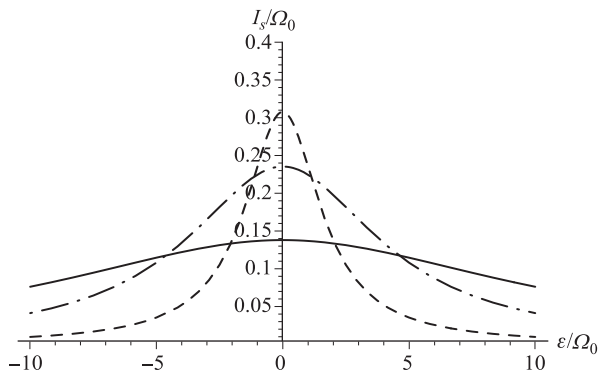
Fig. 13 Electron current through the double-dot, Eq. (126), for \Gamma_L = \Gamma_R = \Omega_0 as a function of the level displacement \epsilon = E_2 - E_1 . The curves correspond to different values of the dephasing rate: \Gamma_d = 0 (dashed), \Gamma_d = 4\Omega_0 (dot-dashed) and \Gamma_d = 16\Omega_0 (solid).
