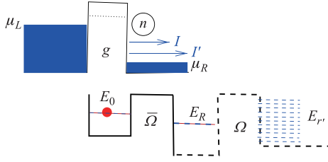
Fig. 18 Measurement of the quantum-well population with a point-contact detector. The current increases whenever the electron leaves the well. n denotes the number of electrons arriving the right lead at time t .
