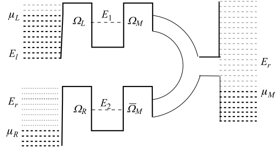
Fig. 7 Two quantum dots, separated by a common reservoir (ballistic channel), as in Fig. 5, where the dots are coupled to the reservoir at spatially close points.
