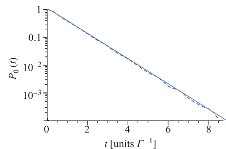
Fig. 16 Probability of finding the particle at its initial state at time t . Dashed line corresponds to periodic chain of N = 250 coupled wells, and solid line shows continuous limit, N \rightarrow \infty , where the density of states is the Lorentzian, Eq. (137).
