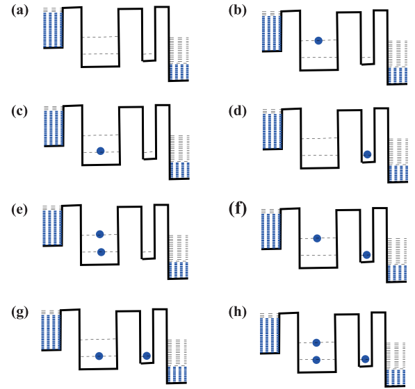
Fig. 4 All possible electron states of the device, shown in Fig. 3: (a) all the levels E_{1,2,3} are empty; (b) the upper level, E_1 , is occupied; (c) the lower level, E_2 , is occupied; (d) the level E_3 is occupied; (e) the levels E_1 and E_2 are occupied; (f) the levels E_1 and E_3 are occupied; (g) the levels E_2 and E_3 are occupied; (h) all the levels E_{1,2,3} are occupied.
