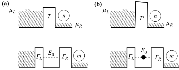
Fig. 8 Ballistic point-contact near quantum-dot. \Gamma_{L,R} are the corresponding tunneling rates. The penetration coefficient of the point-contact is T for the empty dot (a) and T' for the occupied dot (b). The indices m and n denote the number of electrons penetrating to the right reservoirs at time t .
