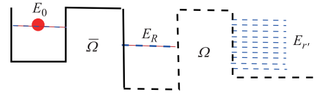
Fig. 17 Tunneling from the left well to continuum through the fictitious well. The level E_R is at the Lorentzian center.
