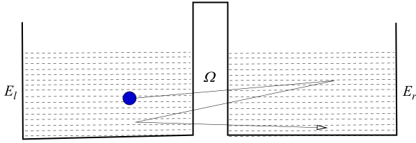
Fig. 9 Motion of a single electron between two reservoirs, described by the tunneling Hamiltonian (82).
