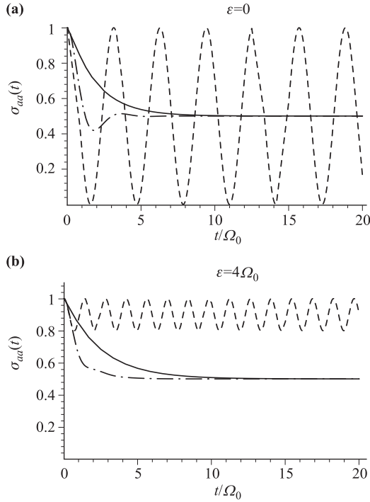
Fig. 11 The occupation of the first well as a function of time, Eqs. (111): (a) the levels are aligned ( \epsilon = 0 ); (b) the levels are displaced ( \epsilon = 4\Omega_0 ). The curves correspond to different values of the dephasing rate: \Gamma_d = 0 (dashed), \Gamma_d = 4\Omega_0 (dot-dashed), and \Gamma_d = 16\Omega_0 (solid).
