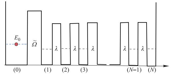
Fig. 15 Tunneling well to a periodic chain of quantum wells with the nearest-neighbor coupling \lambda .
