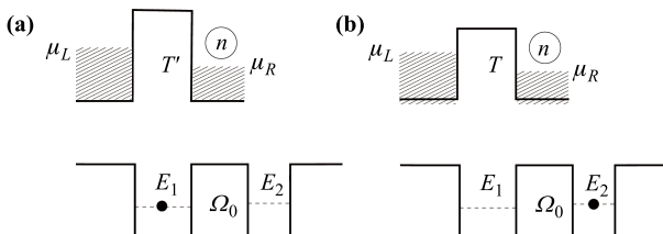
Fig. 10 Electron oscillations in the double-well. The penetration coefficient of the point-contact varies from T' to T when an electron occupies the left well (a) or the right well (b), respectively. The index n denotes the number of electrons accumulated in the collector at time t .
