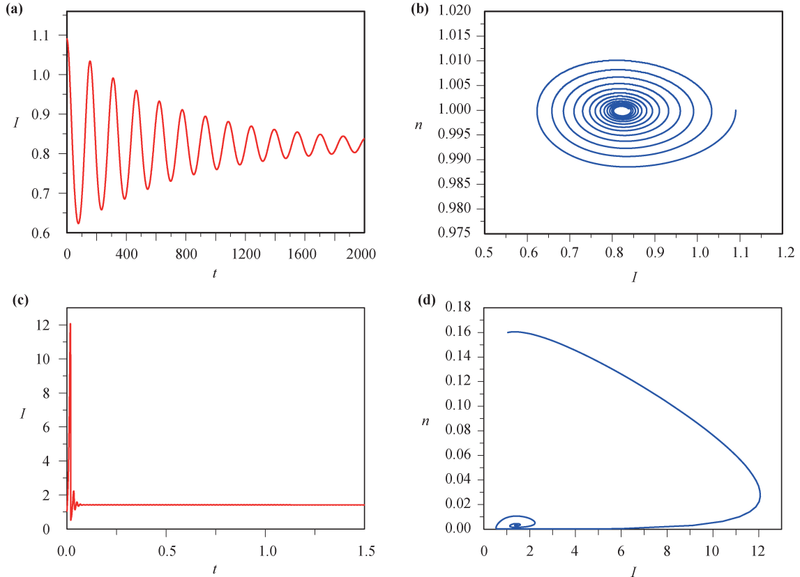
Fig. 4 Solution of the two-variable limits of three-variable rate equations for GNR-array nanolaser. (a), (b) Solution of Eqs. (32) and (33) with I(t = 0) = I_{ss} + 0.1 and G(0) = G_{ss} = 1 . (c), (d) Solution of Eqs. (34) and (35) with I(t = 0) = I_{ss} + 0.1 and n(0) = n_{ss} = 0.15 . The values of the fixed parameters are g = 1.25 , B = 10^3 , and h = 10^{-3} . All variables are dimensionless. Time is normalized by the photon lifetime.
