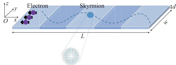
Fig. 1 Schematic diagram of the system under consideration. A chiral ferromagnetic film with spatially modulated Dzyaloshinskii-Moriya interaction is placed in the x - y plane. Spin-polarized electrons are injected to drive the motion of the magnetic skyrmion in the film. L : Length; w : Width; d : Thickness.
