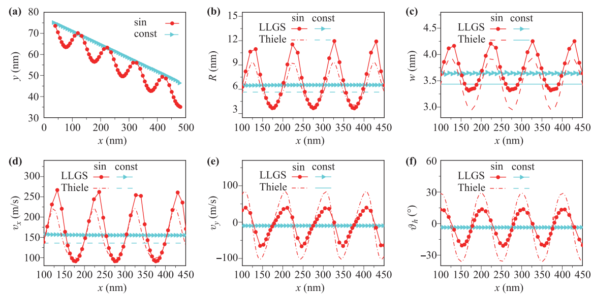
Fig. 4 (a) The trajectory of the skyrmion in the x - y plane of the film; (b) the location-dependent skyrmion radius R ; (c) the location-dependent skyrmion wall width w ; (d, e) the location-dependent velocity components v_x and v_y of the skyrmion; (f) the location-dependent Hall angle \vartheta_H of the skyrmion. LLGS: Micromagnetic simulation based on LLGS equation (2); Thiele: Theoretical results based on Thiele equation. sin: D is sinusoidally modulated as 3.5 + 0.5 \sin(2\pi x/100) mJ/m 2 for x \in [0, 500] nm; const: D takes constant value 3.5 mJ/m 2 for comparison.
