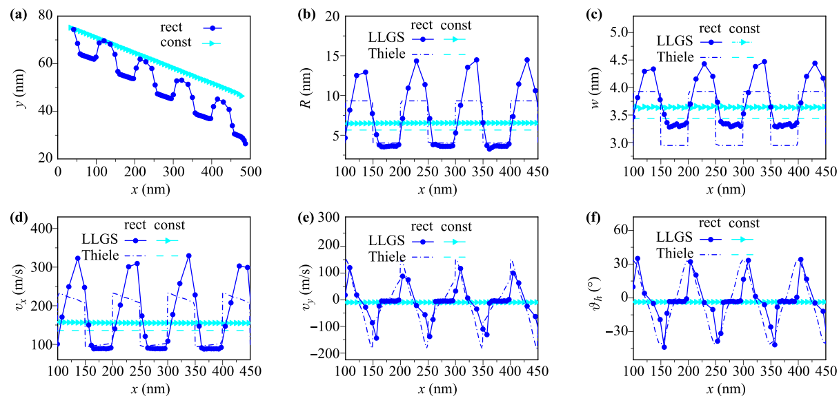
Fig. 5 (a) The trajectory of the skyrmion in the x - y plane of the film; (b) the location-dependent skyrmion radius R ; (c) the location-dependent skyrmion wall width w ; (d, e) the location-dependent velocity components v_x and v_y of the skyrmion; (f) the location-dependent Hall angle \vartheta_H of the skyrmion. LLGS: Micromagnetic simulation based on LLGS equation (2); Thiele: Theoretical results based on Thiele equation. rect: D takes the values 4 \text{ mJ/m}^2 or 3 \text{ mJ/m}^2 alternately per 50 \text{ nm} for x \in [0, 500] \text{ nm} ; const: D takes constant value 3.5 \text{ mJ/m}^2 for comparison.
