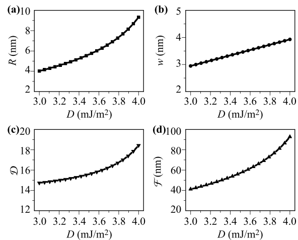
Fig. 2 (a, b) The dependence of the radius R and wall width w of the skyrmion on the DMI strength D according to the model in Ref. [45]. (c, d) The integrals \mathcal{D} defined in Eq. (10) and \mathcal{F} defined in Eq. (11) as functions of D . We have set A = 15 pJ/m and K_u = 0.8 MJ/m 3 in the calculations.
