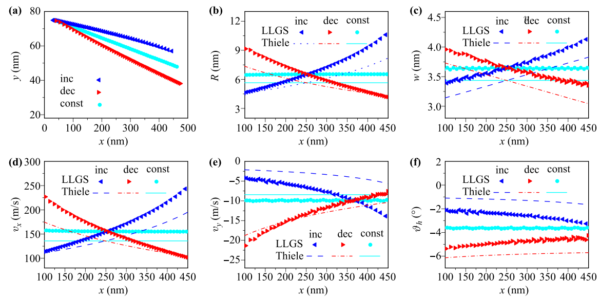
Fig. 3 (a) The trajectory of the skyrmion in the x - y plane of the film; (b) the location-dependent skyrmion radius R ; (c) the location-dependent skyrmion wall width w ; (d, e) the location-dependent velocity components v_x and v_y of the skyrmion; (f) the location-dependent Hall angle \vartheta_H of the skyrmion. LLGS: Micromagnetic simulation based on LLGS equation (2); Thiele: Theoretical results based on Thiele equation. inc: D increases from 3 to 4 mJ/m 2 for x \in [0, 500] nm; dec: D decreases from 4 to 3 mJ/m 2 for x \in [0, 500] nm; const: D takes constant value 3.5 mJ/m 2 for comparison.
