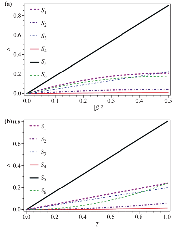
Fig. 4 The relationships of the success probabilities of hyperdistillation schemes vs parameters of less-entangled state. (a) The success probabilities of hyperdistillation schemes vs |\beta|^2 with T_1 = 0.9 and T_2 = 0.8 . (b) The success probabilities of hyperdistillation schemes vs transmission coefficient T_1 = T_2 = T with |\beta|^2 = 0.4 .
