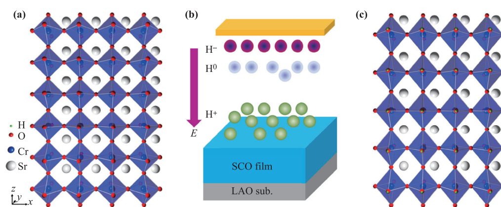
Fig. 1 Schematic views of (a) perovskite SCO with a cubic crystal structure which are formed by edge-sharing \text{CrO}_6 octahedra surrounding by \text{Sr} cations, (b) the low-energy hydrogen plasma implantation process with an applied dc bias to provide a dominant accumulation of protons near the film surface, and (c) the HSCO crystal structure after hydrogen plasma implantation with a lattice expansion of the out-of-plane lattice constant.
