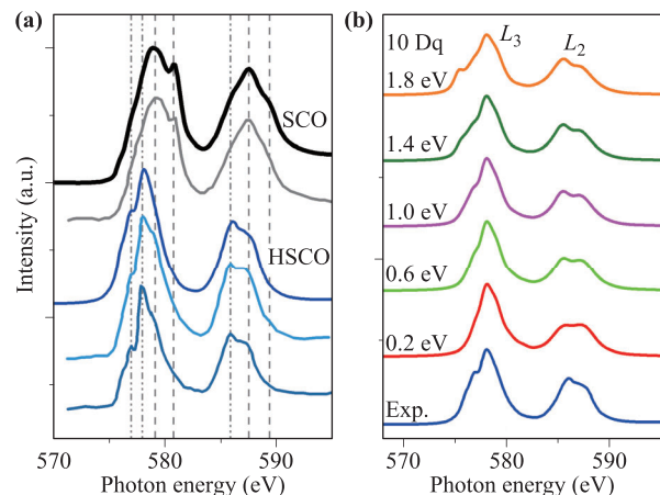
Fig. 4 (a) X-ray absorption spectra at Cr L_{23} -edge for the measured SCO sample, the SCO thin film reported in literature, the measured HSCO film after hydrogen plasma implantation, the measured SrCrO 2.8 thin film with oxygen deficiencies and the LaCrO 3 thin film from top to bottom [33, 34]. (b) Isotropic spectra with different crystal field splitting energies 10 Dq from 0.2 eV to 1.8 eV obtained from CI calculations in comparison with the experimental measured absorption spectrum for HSCO films.
