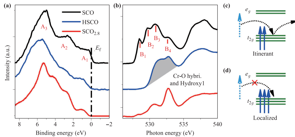
Fig. 5 (a, b) The valence band XPS spectra and O K -edge absorption spectra for SCO film, HSCO film after hydrogen plasma implantation and oxygen deficient SCO 2.8 film. Schematic illustrations of the electronic configurations for (c) pristine SCO and (d) proton-doped HSCO systems in the ionic limit.
