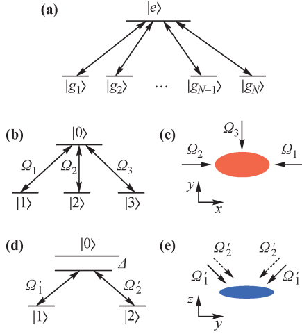
Fig. 9 Schematic of atom-laser interaction. (a) Multi-pod configuration. An atomic state |e\rangle is coupled to N different atomic states |g_j\rangle ( j = 1, \dots, N ) by N resonant laser fields. (b) and (c) Atoms with tripod-level configuration ( N = 3 ) interacting with three laser beams characterized by the Rabi frequencies \Omega_1 , \Omega_2 and \Omega_3 . (d) and (e) Atoms with \Lambda -level configuration interacting with laser beams characterized by the Rabi frequencies \Omega'_1 , \Omega'_2 and a large detuning \Delta .
