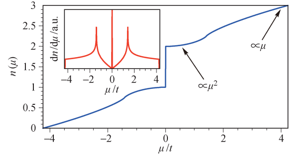
Fig. 7 The number of atoms n per unit cell in \mathcal{T}_3 OLs at zero temperature as a function of \mu/t . Inset: density of states, dn/d\mu , versus \mu/t . Reproduced from Ref. [48], Copyright © 2009 the American Physical Society.
