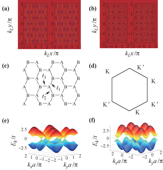
Fig. 1 The honeycomb OLs. (a) and (b) The contours with three potentials described in Eq. (1). The minima of the potentials are denoted by the solid dots. All V_j^0 are the same in (a), and V_1^0 = V_2^0 = 0.91V_3^0 in (b). (c) Decomposition of the hexagonal lattice as two triangular sublattices A and B with anisotropic tunnelling. (d) The Brillouin zone of the hexagonal lattice. The dispersion relations are shown in (e) for \beta = 1 (gapless state) and (f) for \beta = 2.5 (gapped state). Reproduced from Ref. [41], Copyright © 2007 the American Physical Society.
