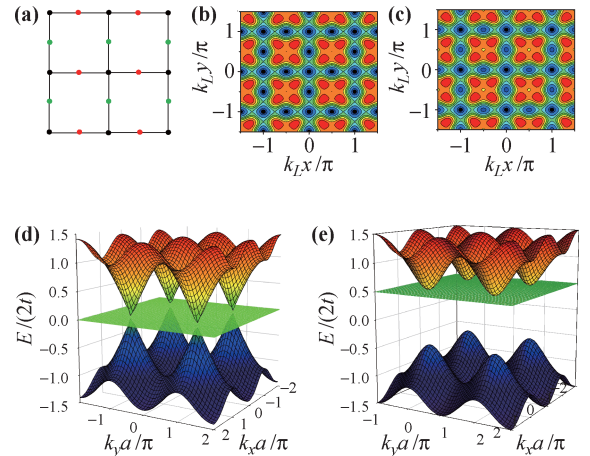
Fig. 3 (a) Schematic illustration of the LCS lattice, energy contour of the optical potential in Eq. (9) with (b) V_1 = 2V_2 and (c) V_1 = 2.2V_2 , and dispersion relation on the LCS lattice with (d) \Delta'_g = 0 and (e) \Delta'_g = t . Reproduced from Ref. [50], Copyright © 2010 the American Physical Society.
