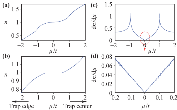
Fig. 6 The number density of atoms n per unit cell of the hexagonal lattice as a function of the chemical potential \mu (corresponding to a re-scaled atomic density profile in a trap) for (a) \beta = 1 , and (b) \beta = 2.5 . A plateau with a width 2\beta - 4 appears for the latter case which corresponds to the case when the chemical potential sweeps inside the energy gap. (c) The derivative dn/d\mu as a function of the chemical potential \mu for \beta = 1 . (d) An enlarged part of dn/d\mu at the vicinity of \mu = 0 . The linearity of the curve shows the linear dispersion relation for the quasiparticles. Reproduced from Ref. [41], Copyright © 2007 the American Physical Society.
