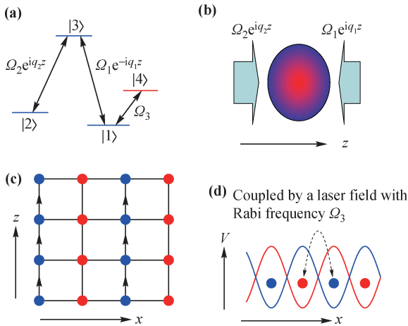
Fig. 4 (a) The atomic levels and the interactions between atoms and laser fields. (b) Schematic representation of the experimental setup with the two laser beams incident on the cloud of atoms. (c) Schematic of the square optical lattice and the designed phase factor (denoted by arrows). (d) The scheme of overlapping the two state-selective optical lattices. Reproduced from Ref. [52], Copyright © 2009 the American Physical Society.
