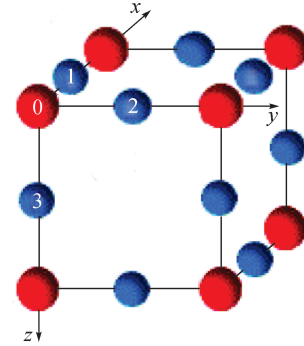
Fig. 5 A crystal cell of the edge-centered cubic lattice and the axis system adapted in this paper. One crystal cell includes four inequivalent lattice sites labeled by 0, 1, 2 and 3, respectively. Reproduced from Ref. [59], Copyright © 2010 the American Physical Society.
