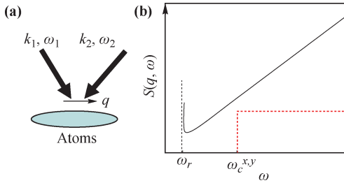
Fig. 8 Schematic of the Bragg scattering. (a) Atoms are illuminated by two laser beams with wave vectors \mathbf{k}_1, \mathbf{k}_2 and frequencies \omega_1, \omega_2 , respectively. (b) The dynamic structure factors S(q, \omega) (not scaled) for the massless Dirac fermions (solid line) and for the massive ones in the non-relativistic limit (dotted line). The experimentally measurable quantities \omega_r and \omega_c^{x,y} give important parameters for the quasiparticles. Reproduced from Ref. [41], Copyright © 2007 the American Physical Society.
