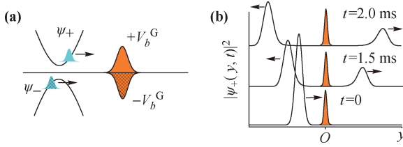
Fig. 13 Schematic representation of the scattering of a BEC. (a) A schematic diagram shows four kinds of scattering events. (b) Normalized density distribution in a scattering process at time t = 0, 1.5 and 2.0 ms. The peaks at y = 0 are the Gaussian barriers.
