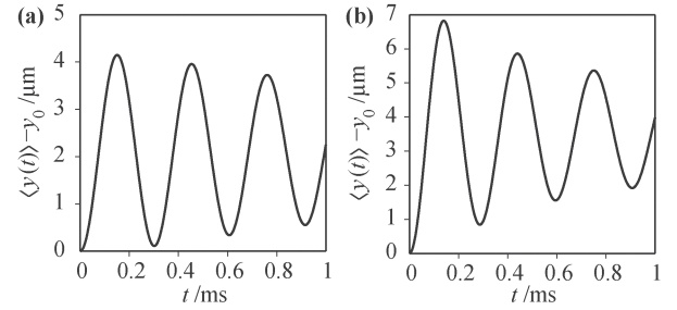
Fig. 10 Zitterbewegung for wave packets of ^7\text{Li} atomic gas with initial wave number k_0 = 0 . (a) \kappa_y = 5.0 \times 10^6 \text{ m}^{-1} , (b) \kappa_y = 1.0 \times 10^7 \text{ m}^{-1} . Other parameters are m = 1.16 \times 10^{-26} , \gamma'_z/\hbar = 10 \text{ kHz} and \delta_l = 10 \mu\text{m} , respectively.
