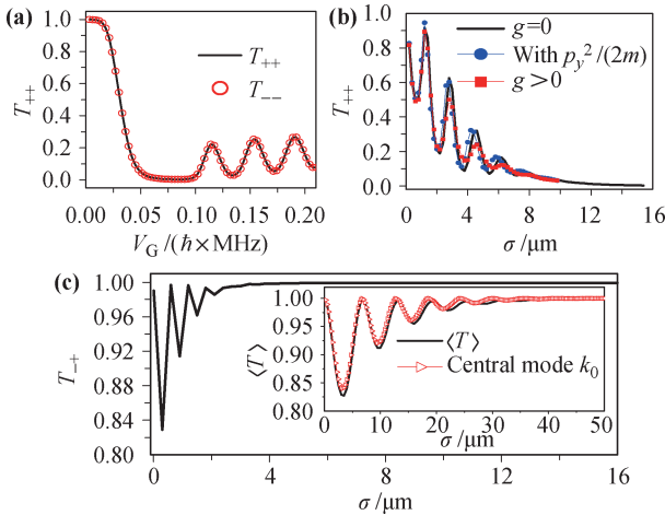
Fig. 14 Klein tunneling of BECs. (a) T_{++} as a function of the potential height V_G with \sigma = 5 \mu\text{m} . The relation T_{++} = T_{--} is confirmed. (b) T_{++} as a function of potential width \sigma with V_G = 0.2 MHz. The tunnelings of a BEC with the classic kinetic energy term and the weak atomic interaction ( N = 2 \times 10^4 , l_\perp = 1.4 \mu\text{m} and a_s = 5a_0 with a_0 being the Bohr radius) are also depicted. (c) T_{++} as a function of potential width \sigma with V_G = 0.2 MHz. In the insert, the transmission coefficient of a plane wave at the central mode k_0 is shown as the line with labels of triangle, while the average transmission coefficient \langle T \rangle of 10^4 atoms is shown as the solid line. The other parameters: l_0 = 10 \mu\text{m} , k_0 = 5.5 \times 10^5 \text{ m}^{-1} , \gamma_z/\hbar = 30 \text{ kHz} , and d = 4(l_0 + \sigma) .
