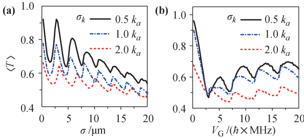
Fig. 12 Klein tunneling of an ensemble of N_a = 10^4 noninteracting atoms. (a) \langle T \rangle as a function of potential width \sigma with \Omega_b^G = 0.8 \text{ MHz} . (b) \langle T \rangle as a function of potential height V_G with \sigma = 10 \mu\text{m} . The black solid line, blue dashed line and red dotted line in both (a) and (b) correspond to the cases of \sigma_k = 0.5, 1.0, 2.0 k_a , respectively. Other parameters are k_a = 1.1 \times 10^6 \text{ m}^{-1} , \kappa_y = 10^7 \text{ m}^{-1} , \kappa_z = 0.8 \times 10^7 \text{ m}^{-1} , frequency \Omega = 10^7 \text{ Hz} , and \Delta = 10^9 \text{ Hz} .
