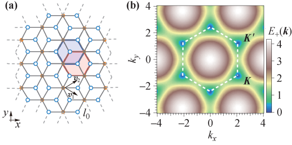
Fig. 2 (a) The \mathcal{T}_3 lattice. It is characterized by translation vectors \mathbf{v}_1 = (3/2; -\sqrt{3}/2)a and \mathbf{v}_2 = (3/2; \sqrt{3}/2)a . Open circles mark the two sublattices A and B, forming a hexagonal lattice. Solid circles mark the hub sites H forming a (larger) triangular lattice. (b) Contour plot of E_+(\mathbf{k}) in units of the hopping energy t , cf. Eq. (7b). The dashed hexagon defines the first Brillouin zone, \mathbf{K} = 2\pi a^{-1}(1/3; -\sqrt{3}/9) and \mathbf{K}' = 2\pi a^{-1}(1/3; \sqrt{3}/9) are two nonequivalent Dirac points. Reproduced from Ref. [48], Copyright © 2009 the American Physical Society.
