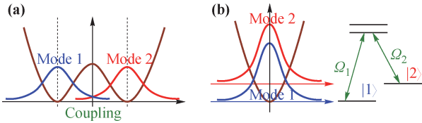
Fig. 4 Schematic diagrams for Bose–Josephson junctions: (a) an external Bose–Josephson junction linked by quantum tunnelling, and (b) an internal Bose–Josephson junction via a two-component BEC linked by Raman fields.
