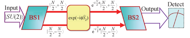
Fig. 10 Schematic diagram for the adiabatic MZ interferometry via a quantized BJJ described by the giant-spin Hamiltonian (61). The input state is an SU(2) coherent spin state along the x -axis. The beam splitters BS1 and BS2 are achieved by the adiabatic processes through the critical point for a bifurcation between normal and self-trapped states.
