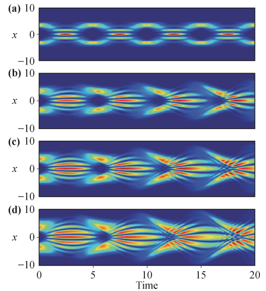
Fig. 3 In-trap interference and nonlinear excitations. The density evolutions |\Phi(x, t)|^2 for \lambda = 0 (linear system), \lambda = 10 , \lambda = 20 and \lambda = 40 are shown in rows (a), (b), (c) and (d), respectively. All initial states are chosen as the ground states for BECs within a double-well potential of parameters \omega = 0.2\pi , d = 1 and B = 40 .
