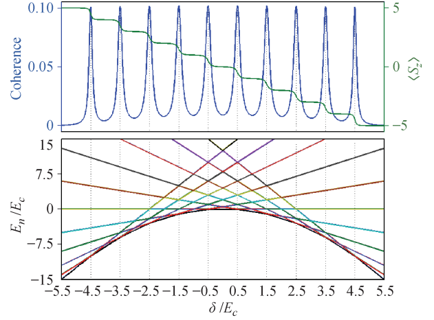
Fig. 9 Interaction blockade, resonant tunneling and energy spectrum for a quantized BJJ of N = 10 and E_c/J = 10 . The first row shows the coherence and the expectation value \langle S_z \rangle versus the asymmetry strength \delta/E_c . The second row shows how E_n/E_c depends on \delta/E_c with E_n denoting the eigenenergy for the n -th eigenstate.
