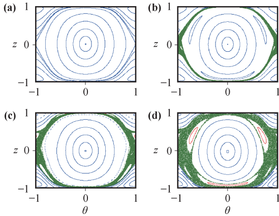
Fig. 7 Poincaré sections for a Bose–Josephson system (18) with J = 1 , E_c = 0.01 , N = 1000 and time-dependent asymmetry \delta(t) = \delta_1 \cos(2\pi t) . (a) \delta_1 = 0.001 , (b) \delta_1 = 1/8 , (c) \delta_1 = 1/4 and (d) \delta_1 = 0.5 .
