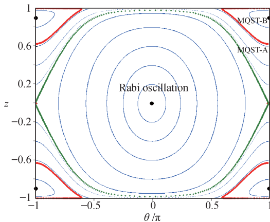
Fig. 6 Rabi oscillations and MQST in a nonlinear Bose–Josephson system described by the Hamiltonian (18) of J = 1 , \delta = 0 , E_c = 0.01 and N = 1000 .
