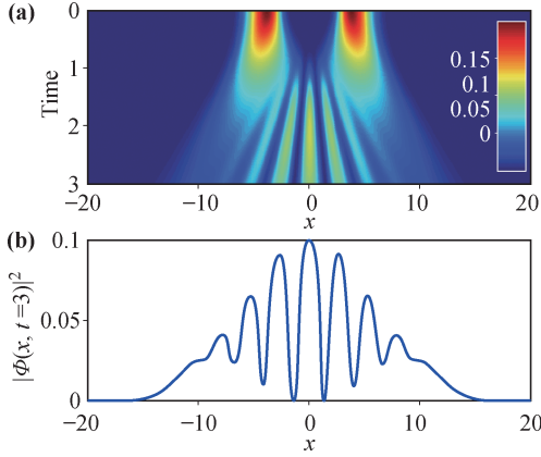
Fig. 2 Interference fringes of two freely expanding condensates. (a) The density evolution |\Phi(x, t)|^2 after switching off the external potential V(x, t) ; and (b) the interference fringe at time t = 3 .
