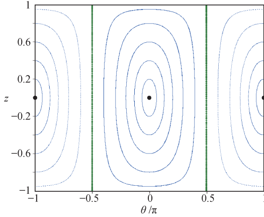
Fig. 5 Rabi oscillations in a linear Bose–Josephson system described by the Hamiltonian (18) of J = 1 , \delta = 0 , E_c = 0 and N = 1000 .
