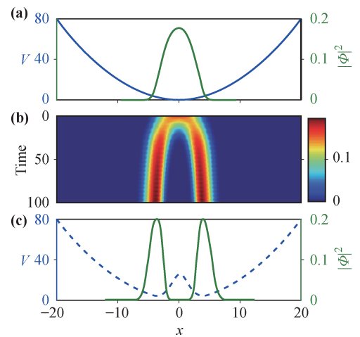
Fig. 1 The splitting process from a single condensate to two condensates. (a) The initial state (green solid curve) at time t = 0 in a harmonic trap (blue dashed curve); (b) the density evolution |\Phi(x, t)|^2 for the splitting process; and (c) the final state (green solid curve) at time t = 100 in a double-well potential (blue dashed curve).
