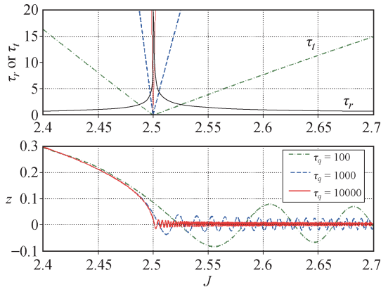
Fig. 8 Dynamics of slow passages through the critical point for the normal-to-MQST transition in a Bose–Josephson system (18) with E_c = -0.01 , N = 1000 and \delta = 0 . The above panel shows how the reaction time \tau_r and the transition time \tau_t depend on the Josephson coupling strength J and the quenching time \tau_q . The bottom panel shows the non-adiabatic dynamics of the fractional population imbalance z .
