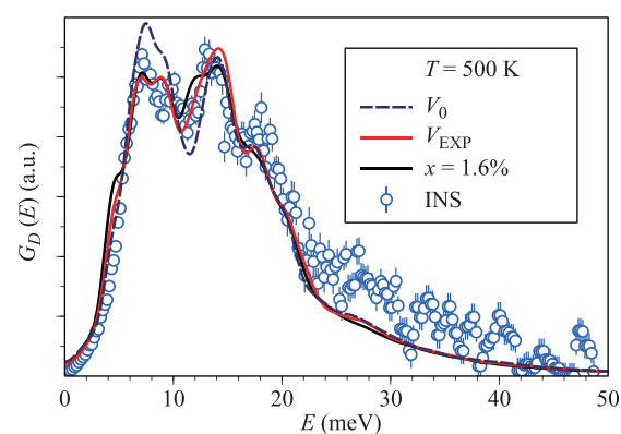
Fig. 2 The INS (open symbols) and AIMD (curves) neutron weighted phonon densities of states of GeTe and \text{Ge}_{1-x}\text{Te} ( x = 1.6\% ) at 500 K. Simulations for the ideal and defected GeTe lattice are performed at the experimental volume ( V_{\text{EXP}} ) determined in our previous NPD measurements [11]. The INS spectra are measured at E_i = 14.34 meV (2.4 Å). The G_D(E) spectra are normalized to unity.
